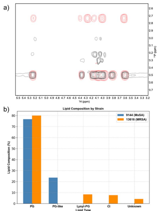
Fig. 4 (a) Overlay of 31 P HSQC spectra of phospholipids extracted from S. aureus ATCC 9144 (red) and S. aureus NCTC 13616 (black); (b) differences in total phospholipid composition between S. aureus ATCC 9144 (blue) and S. aureus NCTC 13616 (orange).
