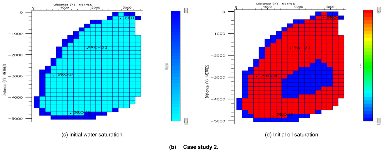
FIGURE 6. (Continued.) Initial pressure, oil, and gas saturation properties under different case studies [6].
