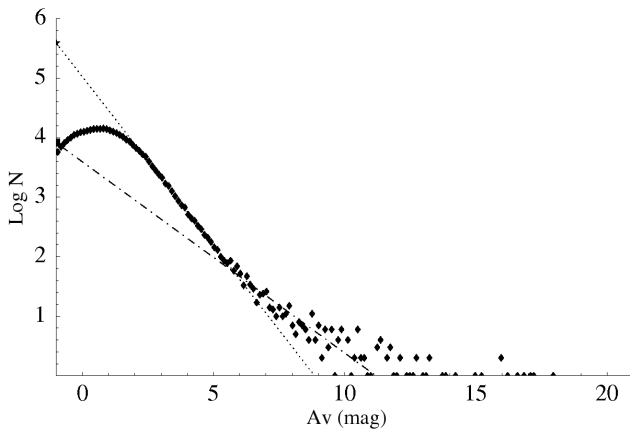
Figure A72. As Fig. A65 but for the cloud Lupus 1, 2.
