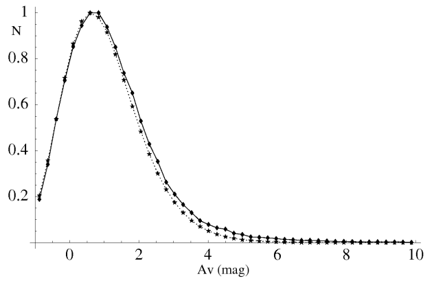
Figure A64. As Fig. A49 but for the cloud Taurus.
