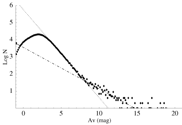
Figure A73. As Fig. A65 but for the cloud Lupus 3, 4, 5, 6.
