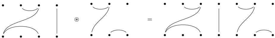
Fig. 4. A horizontal concatenation.
