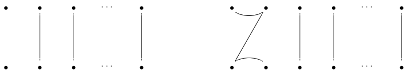
Fig. 3. The non-Coxeter generators p_1 and p_{1,2} of P_r(\delta) .
