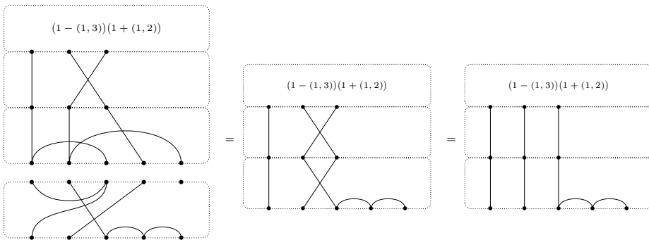
Fig. 8. The product c_{(2,1)}^*(2, 3) d_\Lambda d_{\Gamma'} shown first in non-canonical form as (1 - (1, 3))(1 + (1, 2))(2, 3)d where \pi_d = (2, 3) and then as a canonical basis element from (3.6) as (1 - (1, 3))(1 + (1, 2))d' where \pi_{d'} = 1 .
