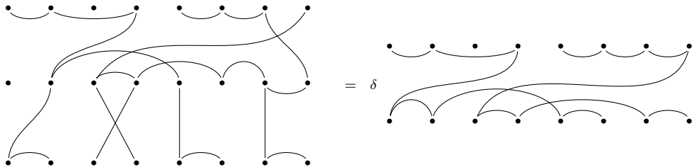
Fig. 2. An example of a product in P_8(\delta) .
