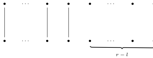
Fig. 5. The idempotent e_l is defined to be \delta^{l-r} times the diagram above having \ell propagating blocks.
