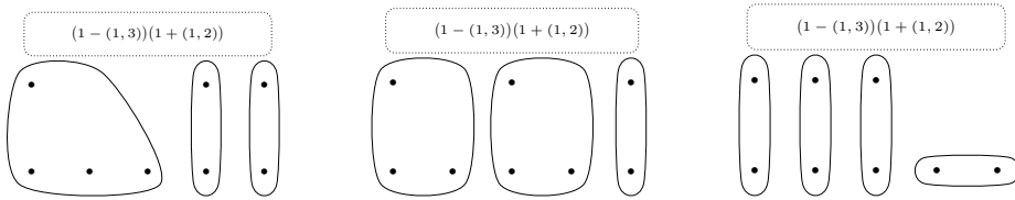
Fig. 28. The generators c_{(2,1)}^* \otimes v_{(\gamma,\varepsilon)} for (\gamma, \varepsilon) equal to ((3, 1^2), \emptyset) and ((2^2, 1), \emptyset) and ((1^3), (2)) respectively. These generate the direct summands, which we denote by M_1 , M_2 , and M_3 of \text{DQ}(\Delta_5(\emptyset^{(2,1)})) .
