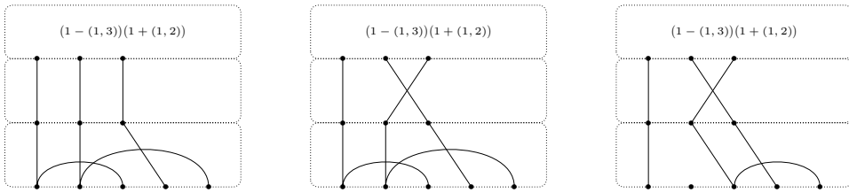
Fig. 6. Three elements shown in the form c_{(2,1)}^* \sigma d_\Lambda in the basis of \Delta_5((2, 1)) from equation (3.6). The bottom halves are (3, 5) -diagrams lying in the basis of V_5(3) , regarding these halves as (5, 5) -diagrams using the identification made at the start of Section 3.4.
