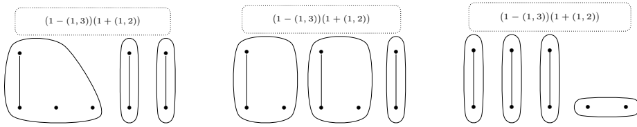
Fig. 29. The generators c_{(2,1)}^* \otimes v_{(\gamma, \epsilon)} for (\gamma, \epsilon) equalling ((1^2, 0), \emptyset) and ((2, 0^2), \emptyset) and (\emptyset, (2)) respectively. The distinguished zero parts for each \gamma \in \mathcal{P}_{(1^3)} are indicated. These diagrams generate the direct summands, which we denote by N_1 , N_2 , and N_3 of \mathrm{DQ}(\Delta_5((1)^{(2,1)})) .
