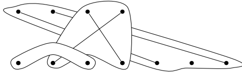
Fig. 19. Another diagram in V_7^0(2^2) . This ramified diagram can be obtained from that of Fig. 18 by acting on the left by ((1, 2), 1\mathfrak{S}_2; (1, 2)) \in \mathfrak{S}_2 \wr \mathfrak{S}_2 . Observe that it cannot be obtained from the ramified diagram of Fig. 18 via a right action.
