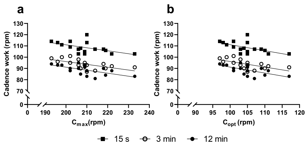
Linear relationships between the C_{\max} (panel a) and C_{\text{opt}} (panel b) to the 15 s, 3 min and 12 min cadence in the CP after accumulated work. C_{\max} – maximum cadence, C_{\text{opt}} – optimum cadence, CP – critical power.
