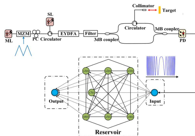
Fig. 1. Schematic diagram of the developed FMCW LiDAR system incorporating time-domain demodulation based on RC algorithm.
