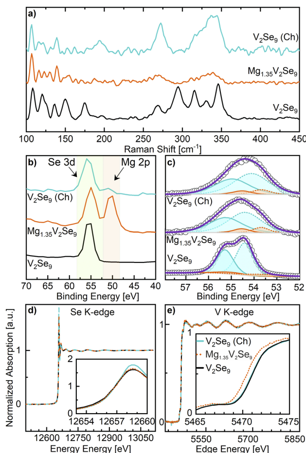
Fig. 5 (a) Ex situ Raman spectroscopy of V_2Se_9 (black), Mg_{1.35}V_2Se_9 (orange) after discharging to 0.8 V and V_2Se_9 after charging (Ch) to 2.2 V (cyan). (b) and (c) XPS spectra of Mg_xV_2Se_9 collected at various stages of discharge/charge. (b) Mg 2p collected at a pass energy of 200 eV and scaled using the Se 3d signal. (c) Se 3d XPS collected at a pass energy of 40 eV. Both Se 3d5/2 and Se 3d3/2 contributions are shown for each Se species: (Se_2)^{2-} (light blue) and Se^{2-} (orange). The sum of orbital contributions is shown as the purple envelope relative to the observed data (black circles). The Se 3d5/2 and 3d3/2 spin–orbit components of each oxidation state were constrained based on relative position, \Delta = 0.86 eV, and intensity ratio = 0.735. The relative areas of Se^{2-}/(Se_2)^{2-} for V_2Se_9 were constrained at 1/8, to reflect the nominal formula V_2Se_9^{5+}(Se_2)^{2-}_4Se^{2-} . Normalized (d) Se K-edge and (e) V K-edge XANES data measured in transmission for V_2Se_9 (black), Mg_{1.35}V_2Se_9 (discharged 0.8 V, orange), and V_2Se_9 (charged 2.2 V, cyan). Inset panels show enlarged profile of the absorption edges at 12 658 eV and 5465 eV, respectively.
