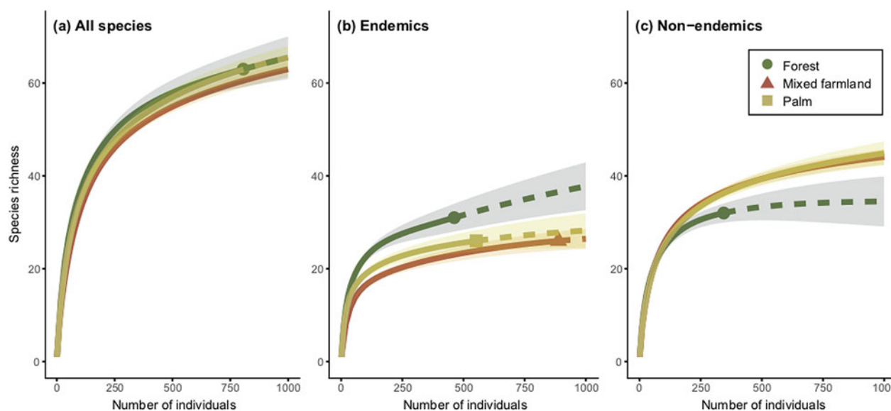
FIG. 2 Rarefied species accumulation curves for bird communities in the forests, coconut palm plantations and mixed farmland of Gorontalo Province, Sulawesi, Indonesia (Fig. 1). We conducted analyses separately for (a) all species, (b) taxa endemic to Sulawesi and the surrounding islands and (c) non-endemic species. We extrapolated the curves (dashed lines) to 1,000 individuals to ensure a consistent sample size for each comparison. We set the confidence intervals (shaded areas) at 84%, which has been demonstrated to be equivalent to a P-value of 0.05 for significant differences (MacGregor-Fors & Payton, 2013).
