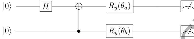
Figure 4: Quantum circuit used in our simulations of rendezvous games on the 3-vertex cycle graph K_3 . From top to bottom, the first qubit represents the quantum sub-system held by Alice and the second qubit that held by Bob.
