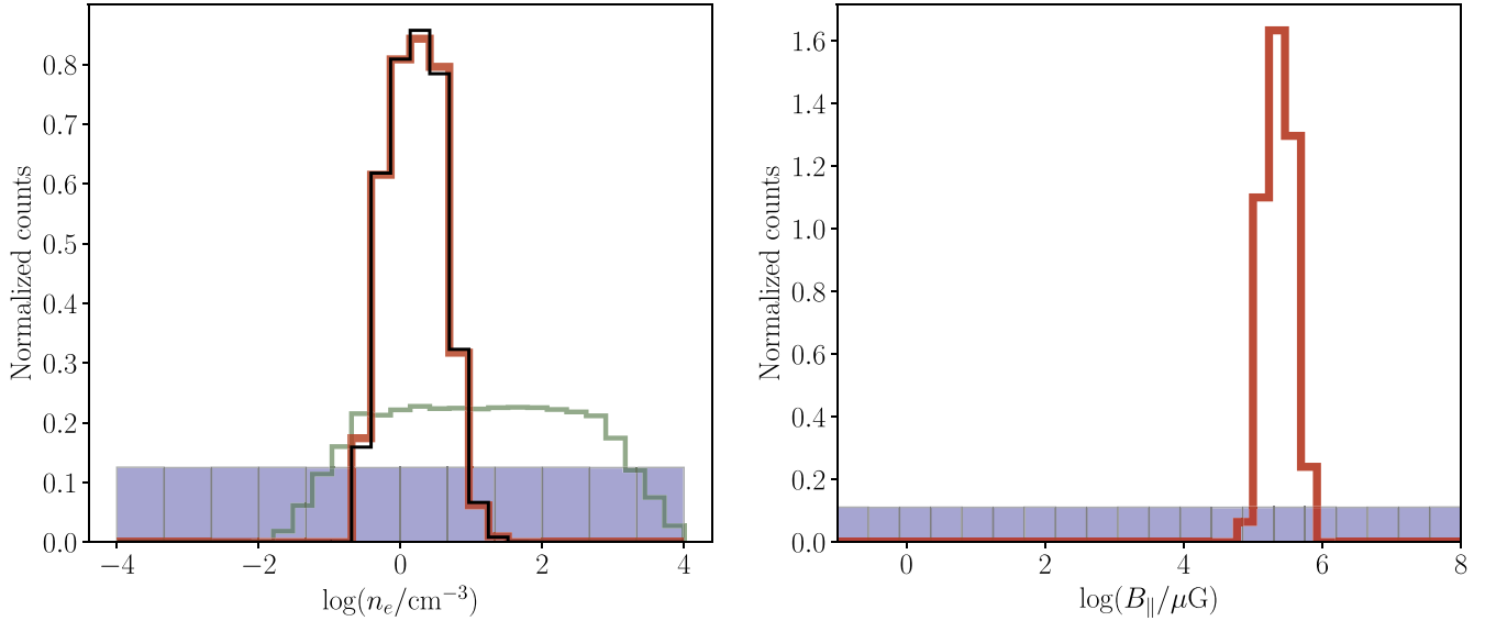
Figure 5. Distributions of n_e (left) and B_{\parallel} (right) under the condition that \nu_{\chi S} and \nu_{rs} match the conditions described in the text. The blue histograms show the uniform distributions of the input parameters. The red histograms show the distributions that satisfy the conditions for both \nu_{\chi S} and \nu_{rs} . In the left panel, the green histogram shows the distribution that matches only the condition for \nu_{\chi S} and the black histogram shows the distribution that matches only the condition for \nu_{rs} . These distributions are not shown on the right, as they would both appear the same as the blue histogram.
