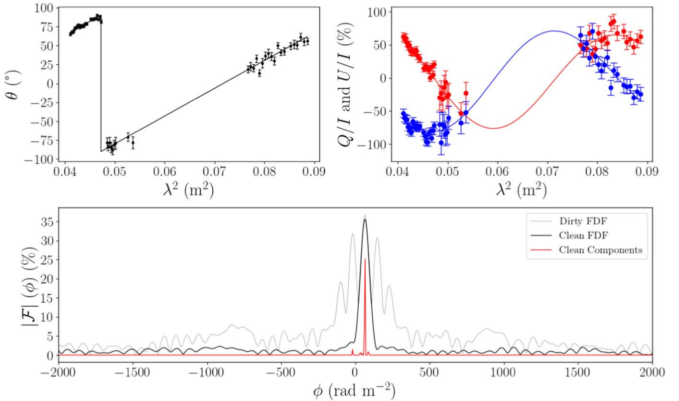
Figure 4. Results of QU fitting and RM clean for ASKAP J173608.2–321635 for the detection in THOR-GC on 2020 April 11. The top left panel shows the polarization angle as a function of \lambda^2 with the model from QU fitting. The top right panel shows Stokes Q (blue) and U (red) as a function of \lambda^2 with the result of QU fitting indicated by the solid lines. The bottom panel shows the dirty FDF in gray, the clean FDF and RM in black, and the clean components from RM clean in red.
