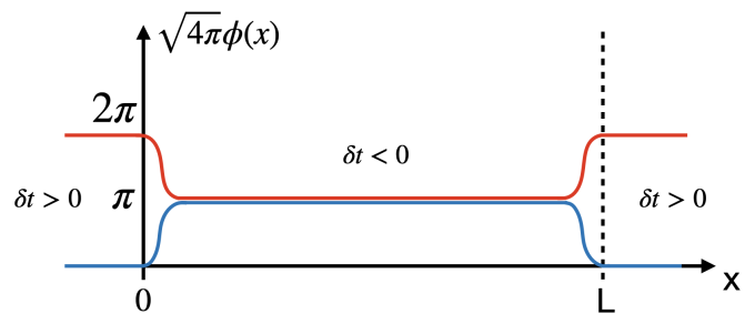
Figure 1: The quasiclassical bosonic ground state for an interface between topologically distinct phases with \delta t > 0 and \delta t < 0 of a non-interacting SSH chain (6). The kinks in the bosonic field \phi(x) at the boundaries correspond to the edge states.
