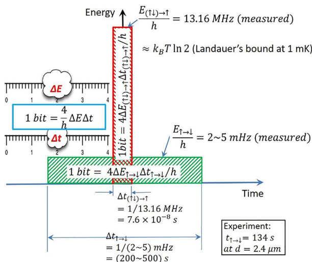
Fig. 6 Heisenberg’s time-energy uncertainty relation (TEUR) [2, 17, 30] is utilized to provide a quantitative definition of information from a measuring perspective: the smallest error in quantifying the product of the measured energy uncertainty ( \Delta E ) and the measured time duration ( \Delta t ) corresponds to 1 bit of information. The two measured energy gaps (13.16MHz and 2 ~ 5mHz) in the spin–spin experiment [27] were utilized as two extreme examples here
