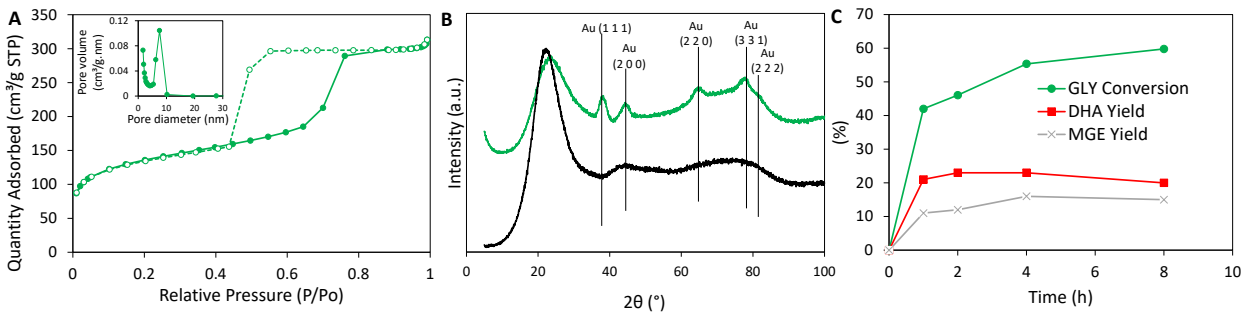
Figure 2: (A) Nitrogen adsorption (plain symbols) and desorption (empty symbols) isotherms of AuSiO 2 . Insert shows BJH pore size distribution analysis obtained from the adsorption isotherm. (B) XRD diffractogram of fresh AuSiO 2 (black) and calcined AuSiO 2 (green) (the detected metallic Au phase corresponds to JCPDS 65-2870). (C) Kinetic study of the oxidation glycerol (GLY) to dihydroxyacetone (DHA) and methyl glycerate (MGE) with AuSiO 2 . Reaction conditions: T = 140°C, p_{air} = 30 bar, 0.25 M glycerol in methanol, and GLY/Catalyst ratio = 2.3 (w/w).
