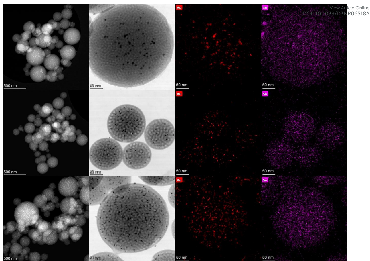
Figure 7: Transmission electron microscope analysis. Respectively from top to bottom: Au(0.5)SnSiO 2 , Au(1)SnSiO 2 and Au(2)SnSiO 2 ; from left to right: HAADF, STEM, STEM-EDX of Au and STEM-EDX of Sn.
