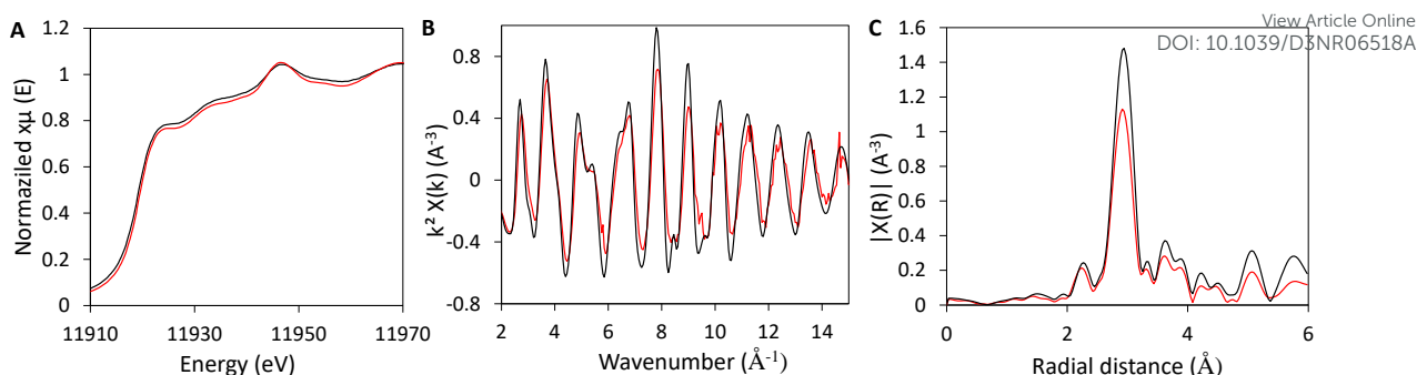
Figure 6: (A) normalized XANES spectra, (B) k^2 \chi(k) EXAFS interference functions and (C) corresponding FTs moduli (phase shift corrected) of Au(1)SnSiO 2 (red curves) and Au foil (black curves). Note that, similarly, the Sn signal was not affected by the presence of Au.
