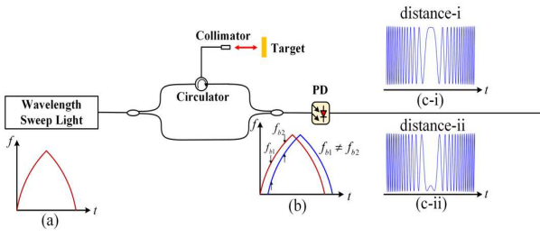
Fig.1. Schematic of the FMCW LiDAR system.
