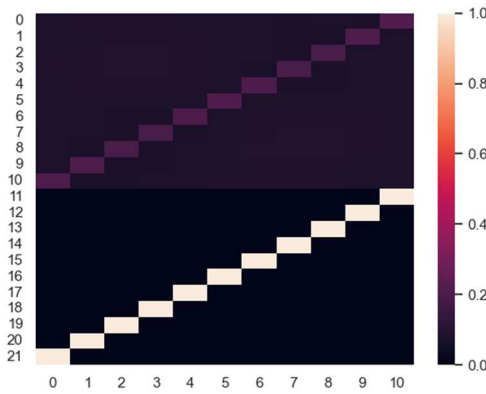
Fig. 4. Results of waveform classification for all the 11 waveforms corresponding to different distances.
