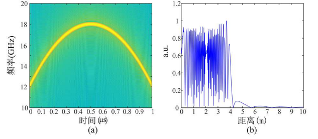
Fig. 2. (a) Instantaneous frequency of FMCW signal. (b) Spectrum broadening due to nonlinearity.
