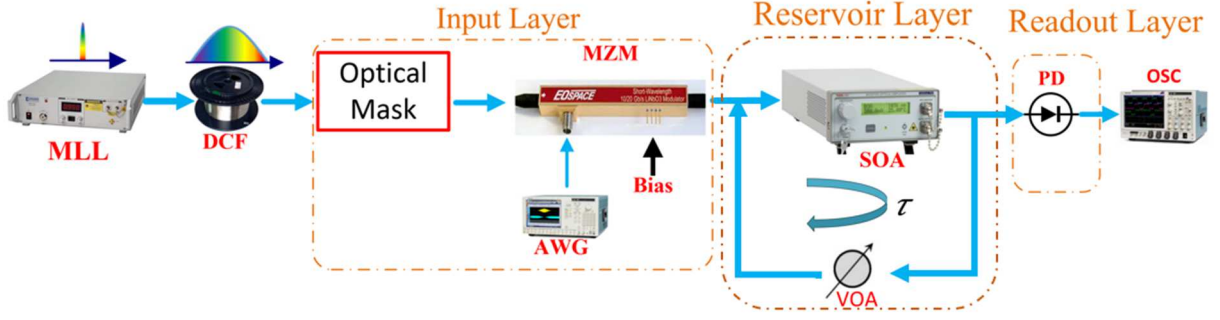
Fig. 1: The schematic of the proposed photonics reservoir computer with an optical mask. MLL: Mode-Locked Laser, DCF: Dispersion Compensating Fibre, MZM: Mach-Zehnder modulator, AWG: Arbitrary Waveform Generator, VOA: Variable Optical Attenuator, SOA: Semiconductor Optical Amplifier, PD: Photodetector, OSC: Oscilloscope.
