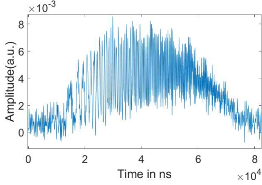
Fig. 2: The measured temporal stretched optical pulse after spectral chirp encoding. A randomly weighted mask can be obtained when uniform sampling is applied at the output layer.
