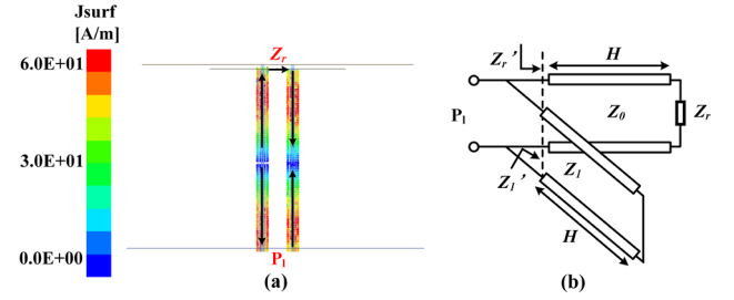
Fig. 7. (a) simulated current distribution on the outer conductor of coaxial cables at 4.4 GHz, (b) equivalent circuit model for the antenna.
