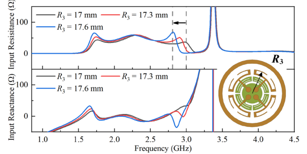
Fig. 12. Simulated input impedance of the proposed antenna under different R_3 .
