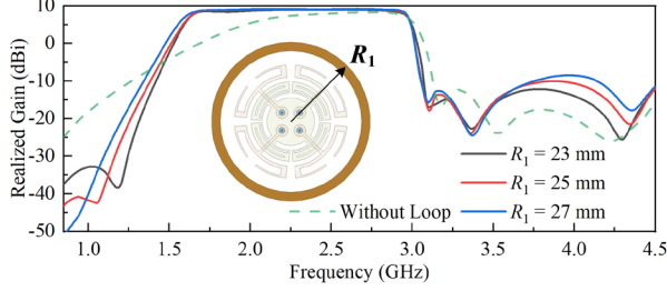
Fig. 9. Simulated realized gains of the proposed antenna under the effect of parasitic loop.
