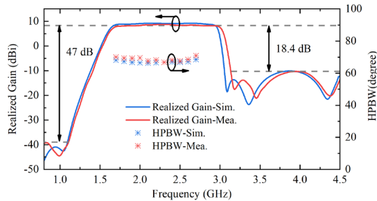
Fig. 14. Measured and simulated realized gains of the proposed antenna.
