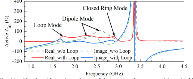
Fig. 11. Simulated input impedance of the proposed antenna with and without parasitic loop.
