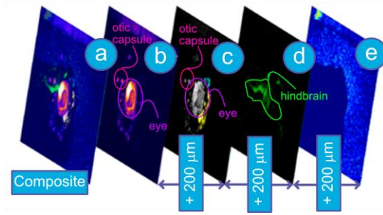
Figure 3. (a) Composite en-face image obtained by merging images collected at 24 axial positions separated by 50 \mu\text{m} . (b)-(e): images showing significant examples of defined brain structures that appear as the focal plane is shifted deeper into the tadpole.
