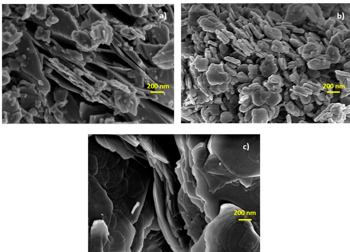
Figure 2. SEM images of (a) Zn-Ti LDH, (b) Zn-Al LDH and (c) Mg-Al LDH.
