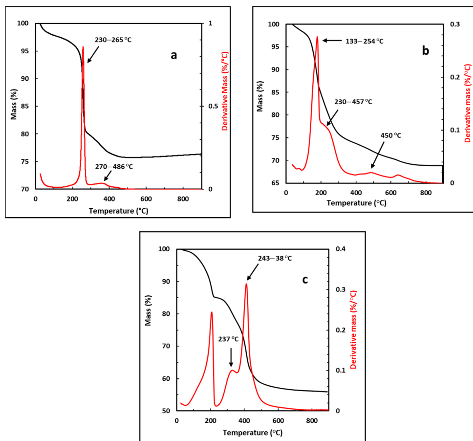
Figure 4. TGA and DTG curves for (a) Zn-Ti LDH, (b) Zn-Al LDH, and (c) Mg-Al LDH.
