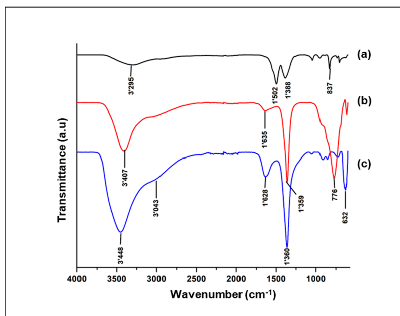
Figure 3. FTIR Spectra of (a) Zn-Ti LDH, (b) Zn-Al LDH and (c) Mg-Al LDH.
