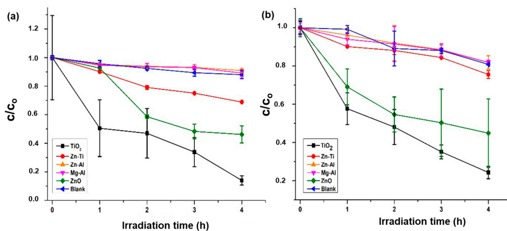
Figure 6. Photodegradation of MB references under (a) 254 nm and (b) 365 nm.
