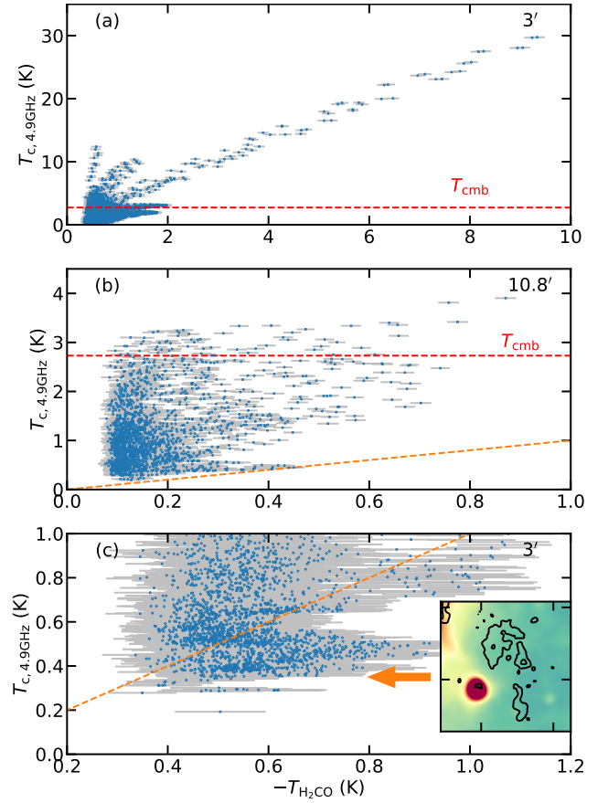
Fig. 12. Comparison between the peak intensities of \text{H}_2\text{CO} absorption and the temperatures of the 4.89 GHz radio continuum emission at an angular resolution of 3' (a) and 10.8' (b). All data points have signal-to-noise ratios of >5 . In both panels, the red dashed line represents the CMB temperature of 2.73 K. (c) Same as panel (a) but zoomed into a narrower intensity range. The panel in the lower right corner is the same as Fig. 5a but zoomed into the region where the absorption dip is greater than the radio continuum temperature. In panels (b) and (c), the orange dashed line marks the equality between \text{H}_2\text{CO} peak absorption and radio continuum temperature. In all panels, the error bars represent a 1\sigma uncertainty.
