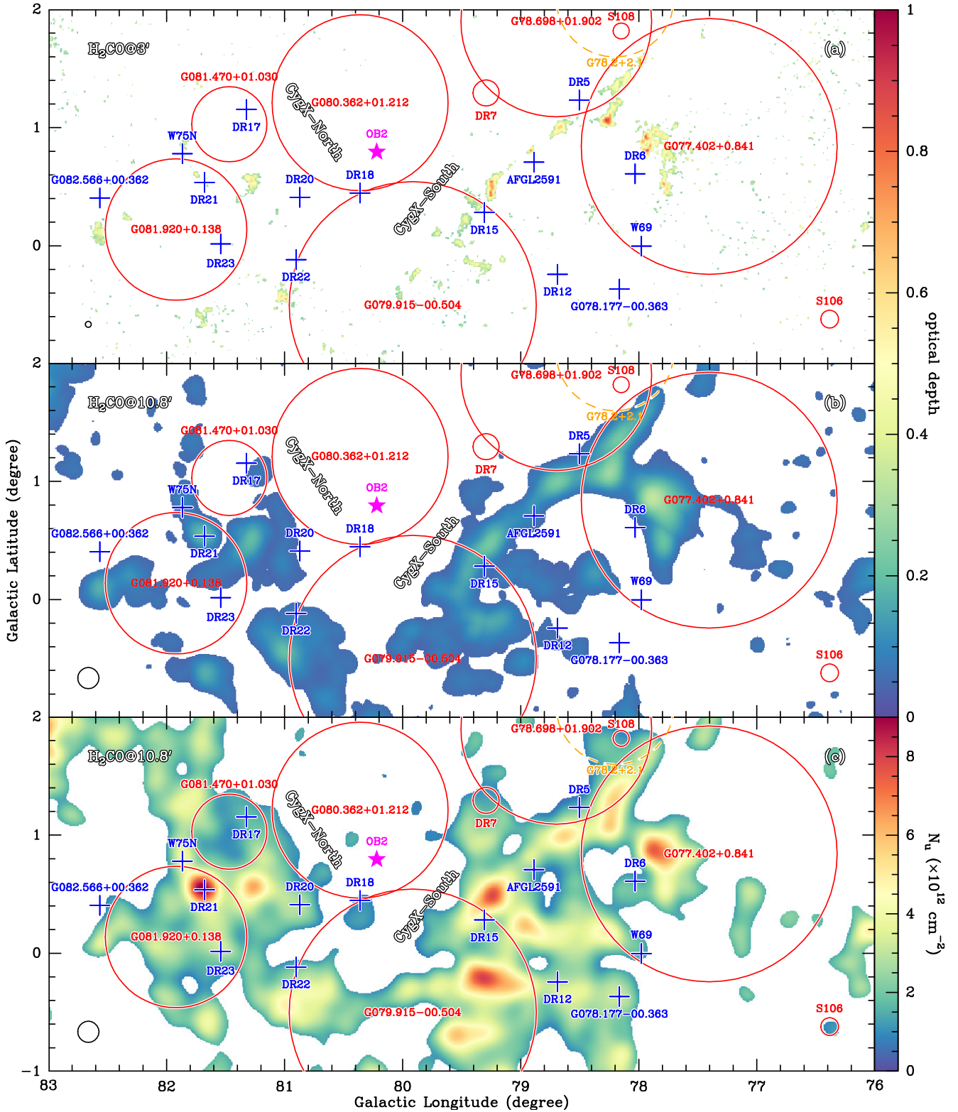
Fig. 6. (a) Distribution of the peak optical depth of the \text{H}_2\text{CO} ( 1_{1,0}-1_{1,1} ) line. The HPBW of the \text{H}_2\text{CO} image is 3' . The color bar represents the peak optical depth. The \text{H II} regions from Anderson et al. (2014) are marked with red solid circles, while SNR G78.2+2.1 is indicated by an orange dashed circle. The blue crosses represent the radio continuum sources and active star-forming objects, and the purple star represents the massive star cluster, Cygnus OB2. (b) Similar to Fig. 6a but the HPBW of the \text{H}_2\text{CO} ( 1_{1,0}-1_{1,1} ) image is 10/8 . (c) Similar to Fig. 6b but for the \text{H}_2\text{CO} column density in the 1_{1,0} level. In all panels, the beam size is shown in the lower left corner.
