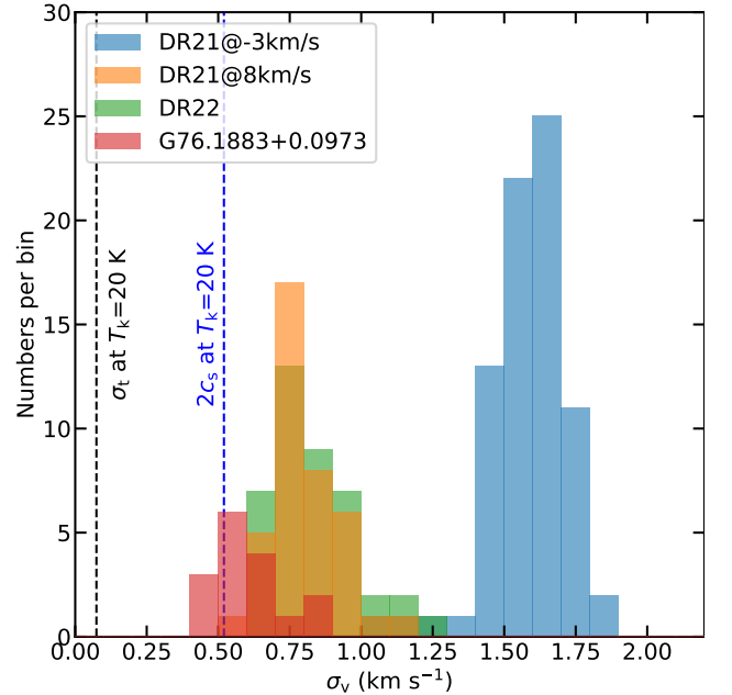
Fig. 11. Histogram of the observed velocity dispersions derived from the VLA+Effelsberg combined \text{H}_2\text{CO} data. The black and blue vertical dashed lines represent the thermal velocity dispersion of \text{H}_2\text{CO} and twice the sonic speed at a kinetic temperature of 20 \text{ K} , respectively.
