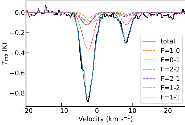
Fig. 3. Observed \text{H}_2\text{CO} ( 1_{1,0}-1_{1,1} ) spectrum at an HPBW of 10'8 toward DR21 (the black solid line) overlaid with the fitted model (the blue solid line). The two velocity components at -3 \text{ km s}^{-1} and 8 \text{ km s}^{-1} correspond to two physically distinct velocity components which arise from the DR21 cloud and its foreground cloud associated with W75N. The fitted HFS components are indicated by the colored dashed lines in the legend.
