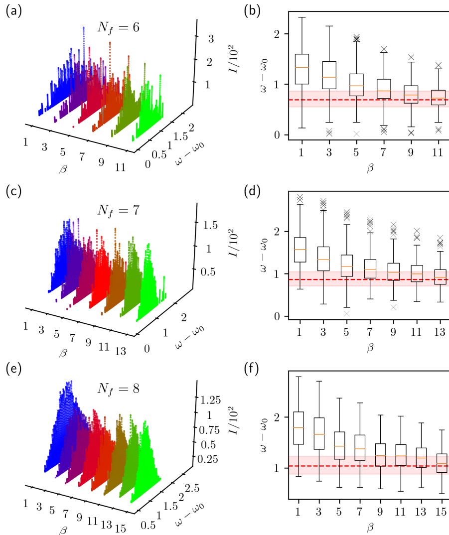
FIG. S4. Approximating the Coulomb structure factor using Yukawa pseudopotentials at \lambda = 0.1 . Structure factor I_{\bar{\rho}}(0, \omega) for the \nu = 1/3 FQH state on a torus, corresponding to the system in Fig. S3(c). (a,c,e) 3D plots showing the scaling of I_{\bar{\rho}}(0, \omega) with truncation parameter \beta \in \{1, 3, \dots, \beta_{\max}\} , where \beta_{\max} is the smallest odd integer greater than (N_{\Phi} + 2)/2 , for (a) N_f = 6 , (c) N_f = 7 , and (e) N_f = 8 . (b,d,f) Box plots showing the spread of I_{\bar{\rho}}(0, \omega) as a function of \beta , for (b) N_f = 6 , (d) N_f = 7 , and (f) N_f = 8 . Outliers are shown explicitly as black crosses. The center and spread for the corresponding exact Coulomb distributions are overlaid in red. The computations were performed with a resolution of \Delta\omega = 10^{-5} , \Delta I = 10^{-5} , and \epsilon = 10^{-4} .
