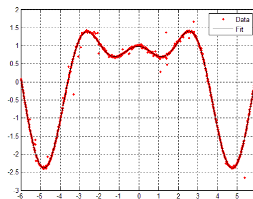
Fig. 2. Data and WN approximation using 8 hidden units.
