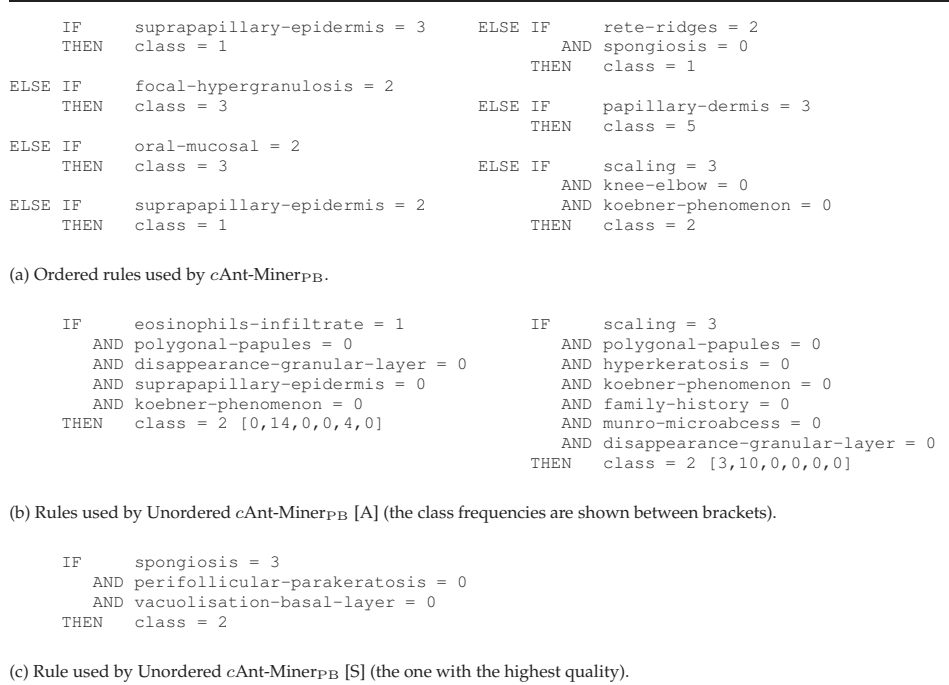
Figure 4: Rules used to classify a particular test example from the dermatology dataset: (a) in cAnt-Miner PB , rules need to be evaluated following their order—rule 7 (bottom rule from the second column) is used only if all previous rules do not classify the example (total of 10 attribute-conditions); (b) Unordered cAnt-Miner PB [A] can make the same prediction using 2 rules (total of 12 attribute-conditions); (c) Unordered cAnt-Miner PB [S] uses only 1 rule (total of 3 attribute-conditions) to make the same prediction.
