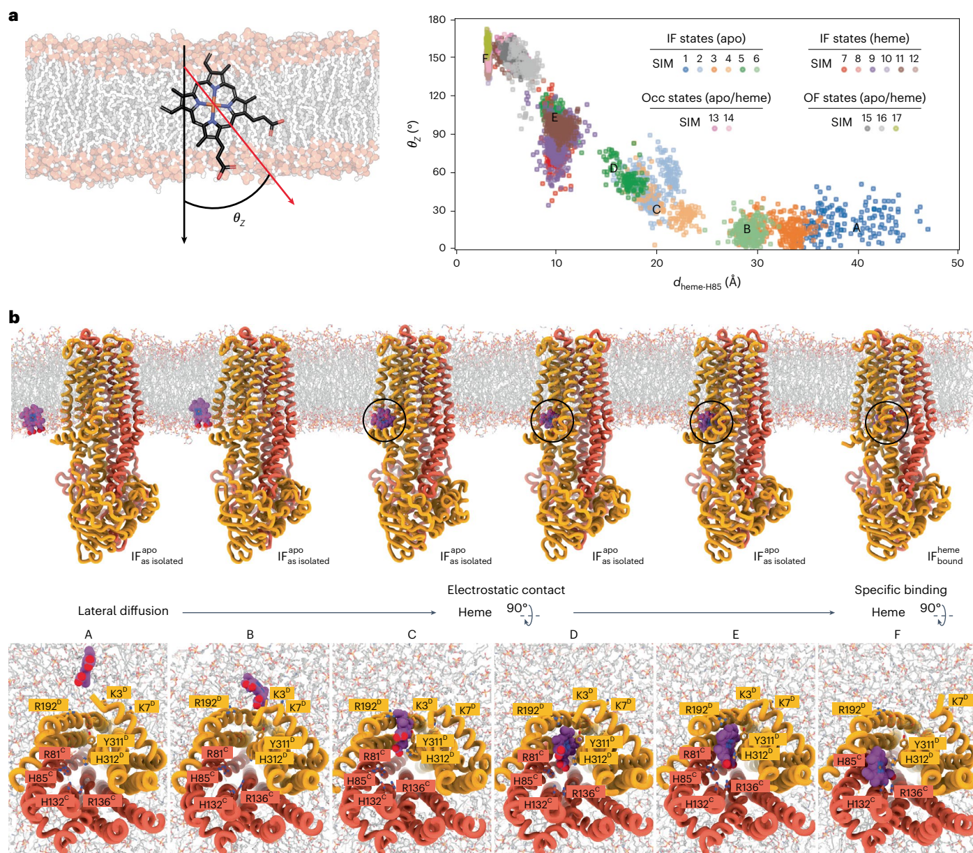
Fig. 4 | Structural dynamics of the heme binding and flipping mechanism.
