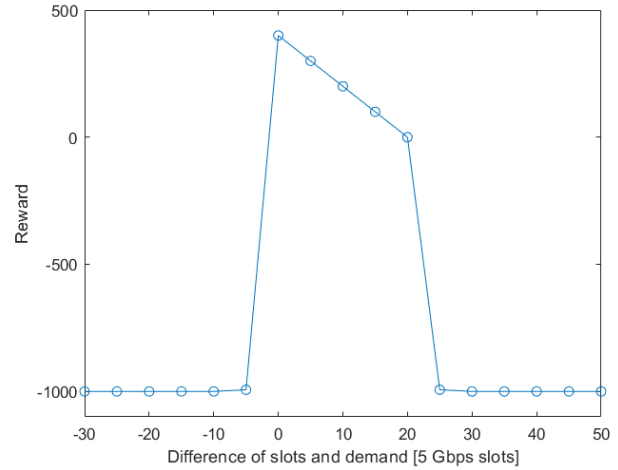
Fig. 6. Reward vs difference of allocated slots and input traffic demand.
