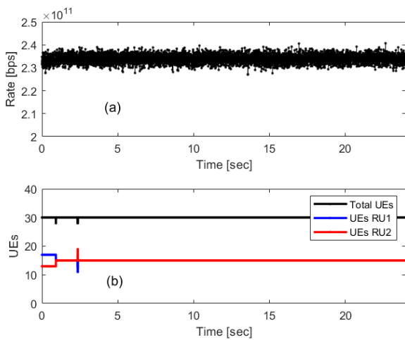
Fig. 11. Controller agent deployment results, total achievable bit rate (a), number of users in RU-groups (b) for RU positions in Figure 5).
