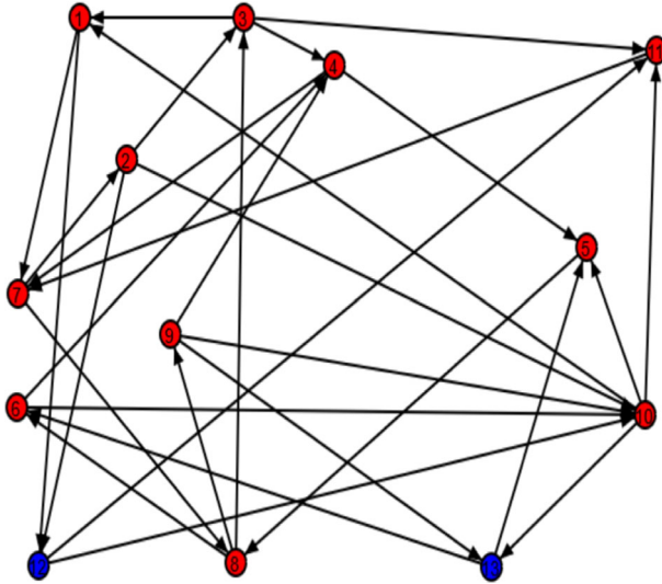
Fig. 4 The initial quiver associated with the extended exchange matrix (2.30)
