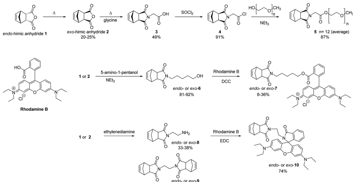
Scheme 1 Monomer synthesis.
