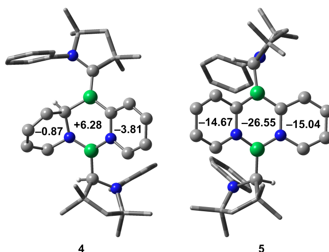
Figure 3. NICS zz (1) values (ppm) of the rings of compounds 4 and 5 at the \omega B97X-D/6-311 + + G(d,p)// \omega B97X-D/6-31G(d,p) level of theory. Selected hydrogen atoms are omitted for clarity. For reference, the NICS zz (1) value of benzene at the same level is -29.75 ppm, while those of anthracene are -25.37 ppm (outer rings) and -35.09 ppm (central ring).
