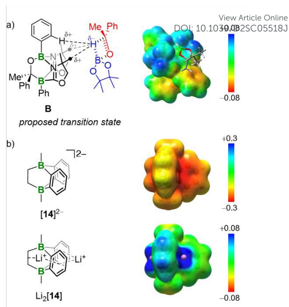
Fig. 3 Comparison of Lewis structures and computed charge densities of a) Kinjo's bicyclic catalyst B and b) compounds [14]^{2-} and \text{Li}_2[14] .
