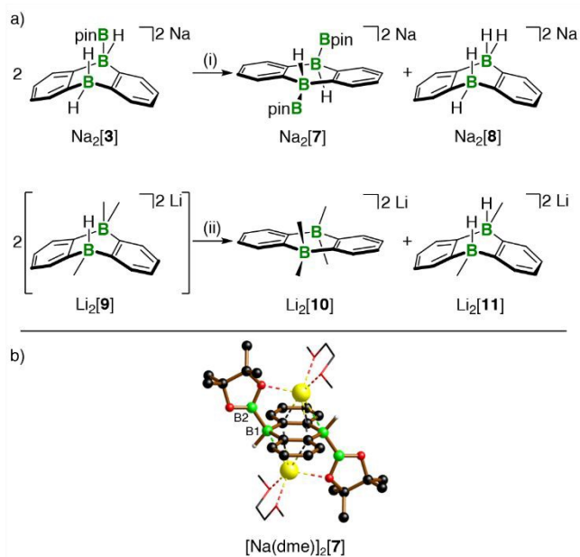
Scheme 3 a) Substituent-redistribution reaction at \text{Na}_2[3] producing \text{Na}_2[7] with two Bpin bonds. Substituent-redistribution reaction at \text{Li}_2[9] leading to the pair of more symmetric compounds \text{Li}_2[10]/\text{Li}_2[11] . b) X-ray-crystallographically derived solid-state structure of the solvate [\text{Na}(\text{dme})_2]_2[7] , featuring two B–Bpin bonds. C-bonded H atoms are omitted for clarity; the dme ligands are shown as wireframes; B: green, C: black, O: red, Na: yellow spheres. (i) DME, room temperature, prolonged storage during crystallization experiments; (ii) THF- d_6 , room temperature.
