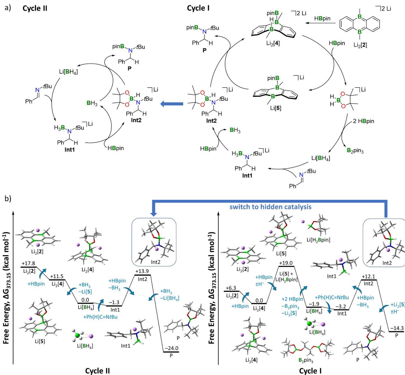
Fig. 4 a) Right: Catalytic Cycle I (hydride shuttle: \text{Li}[\text{H}_2\text{Bpin}] ). Left: Catalytic Cycle II, hidden catalysis (hydride shuttle: \text{Li}[\text{BH}_4] ). b) Right: Free energy diagram for catalytic Cycle I. Left: Free energy diagram for hidden catalysis Cycle II including \text{BH}_3 , thf/ \text{Li}[\text{BH}_4] . Energies are referenced to the starting point of the respective cycle. Level of theory: SMD(solvent=THF)/ \omega B97XD/6-311++G(d,p) from optimized structures at SMD(solvent=THF)/ \omega B97XD/6-31+G(d,p). Explicit thf molecules are omitted for clarity.
