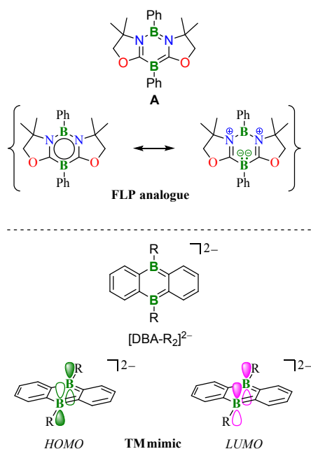
Fig. 1 Top: 1,3,2,5-Diazadiborinine A can be regarded as B(I)/B(III) mixed-valence system, which activates substrate molecules in a similar manner to LB/LA-FLPs. Bottom: The frontier orbital symmetries of the 9,10-dihydro-9,10-diboraanthracene (DBA) dianion [\text{DBA-R}_2]^{2-} allow concerted transition metal-like (TM-like) reactions.
