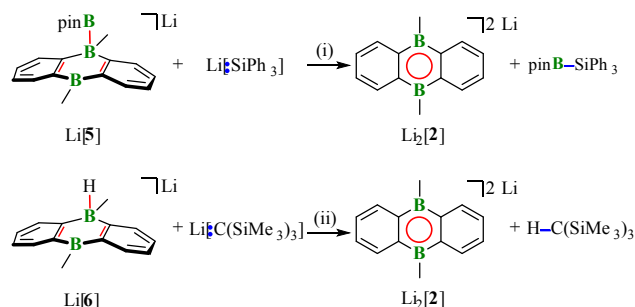
Scheme 2 Reactions of \text{Li}[\mathbf{5}] and \text{Li}[\mathbf{6}] with an Si-centered nucleophile and a C-centered Brønsted base to demonstrate transfer of [\text{Bpin}]^+ and \text{H}^+ along with the suitability of [\mathbf{2}]^{2-} as leaving group. (i) THF- d_6 , room temperature, overnight; (ii) THF- d_6 , 115 °C, 35 h.
