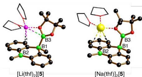
Fig. 2 X-ray-crystallographically derived solid-state structures of the solvates [\text{Li}(\text{thf})_2][\mathbf{5}] and [\text{Na}(\text{thf})_2][\mathbf{5}] , featuring one B–Bpin bond. C-bonded H atoms are omitted for clarity; the thf ligands are simplified as wireframes; Li: pink, B: green, C: black, O: red, Na: yellow spheres.
