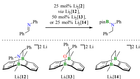
Scheme 4 Crossover experiment to demonstrate that hydroboration of \text{Ph}(\text{H})\text{C}=\text{NPh} with \text{HBpin} can be mediated not only by \text{Li}_2[2] (actual catalyst: \text{Li}_2[12] ), but also by pre-formed \text{Li}_2[13] or \text{Li}_2[14] without generating \text{Ph}_2(\text{H})\text{C}-\text{OBpin} or \text{H}_3\text{C}-\text{CH}_2\text{Bpin} as crossover side product, respectively ( \text{THF-}d_8 , room temperature). Note that the high catalyst loadings were used for the sole purpose of being able to detect any catalyst degradation or trace formation of crossover products by NMR spectroscopy.
