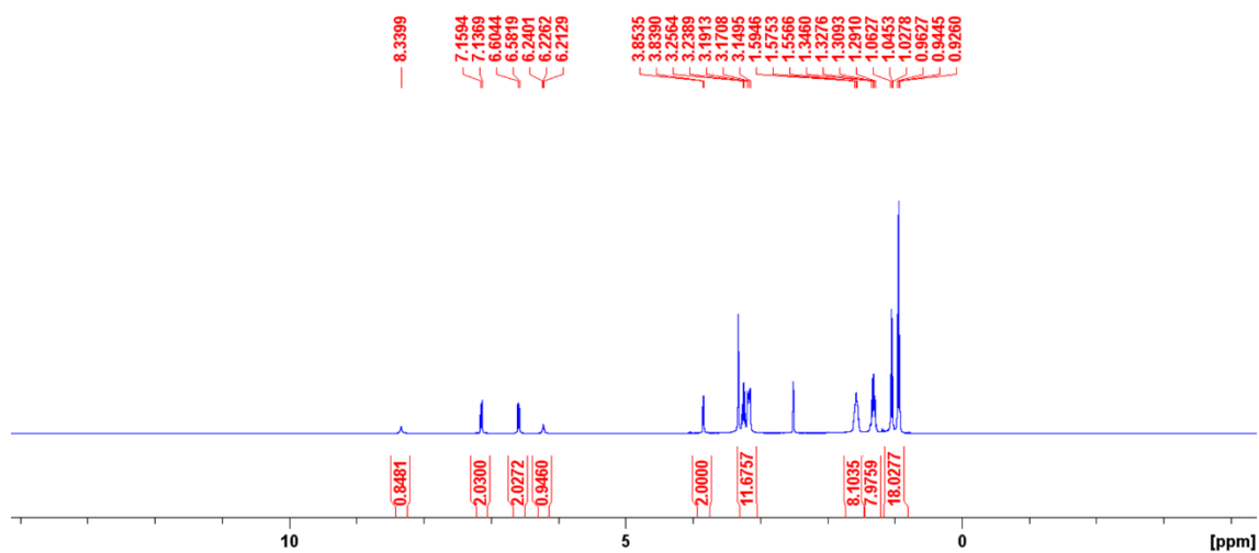
Figure S3 - 1 H NMR of compound 2 in DMSO- d 6 conducted at 298 K.
