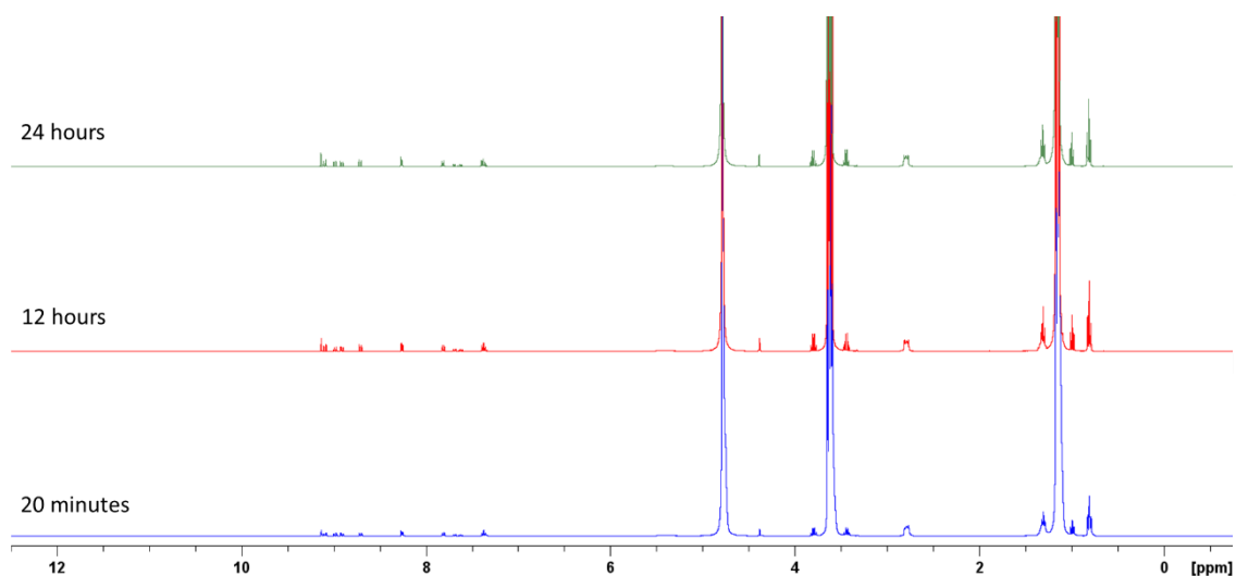
Figure S47 - Zoomed in ^1\text{H} NMR spectrum with a delay ( d_1 = 60 s) of Co-formulation h (5.56 mM) in \text{D}_2\text{O}/5.0\% EtOH. Comparative integration indicated 72% of sample has become NMR silent 20 minutes after the addition of 8-Hydroxypyrene-1,3,6-trisulfonic acid trisodium salt, 72% of the sample has become NMR silent after 12 hours and 72% has become NMR silent after 24 hours.
