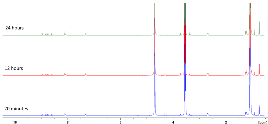
Figure S46 - Zoomed in ^1\text{H} NMR spectrum with a delay ( d_1 = 60 s) of Co-formulation g (5.56 mM) in \text{D}_2\text{O}/5.0\% EtOH. Comparative integration indicated 50% of sample has become NMR silent 20 minutes after the addition of 8-Hydroxypyrene-1,3,6-trisulfonic acid trisodium salt, 50% of the sample has become NMR silent after 12 hours and 50% has become NMR silent after 24 hours.
