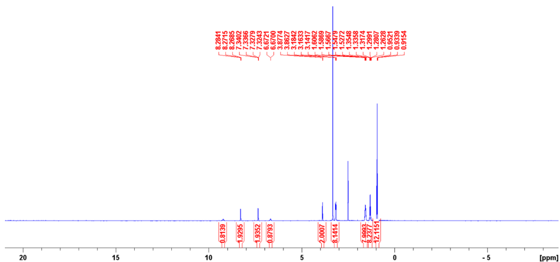
Figure S4 - 1 H NMR of compound 3 in DMSO- d 6 conducted at 298 K.
