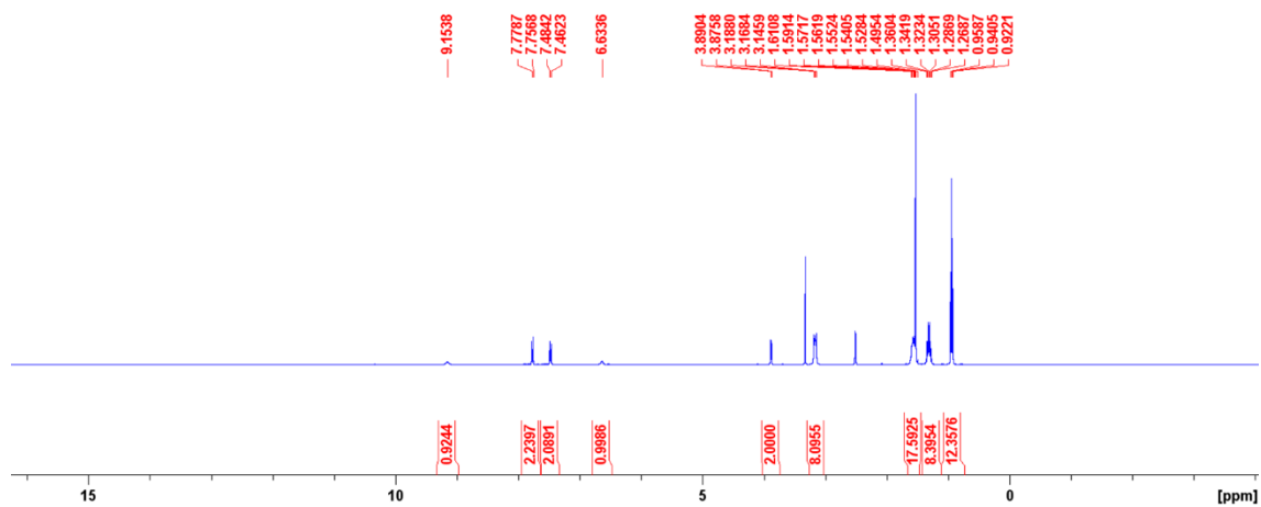
Figure S6 - 1 H NMR of compound 4 in DMSO- d 6 conducted at 298 K.
