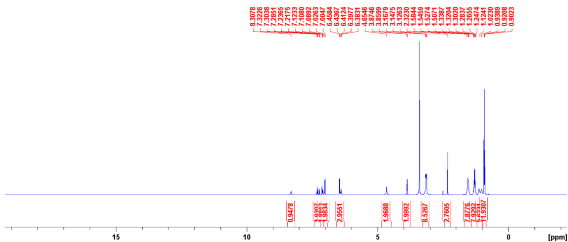
Figure S20 - 1 H NMR of compound Co-formulation i in DMSO- d 6 conducted at 298 K.
