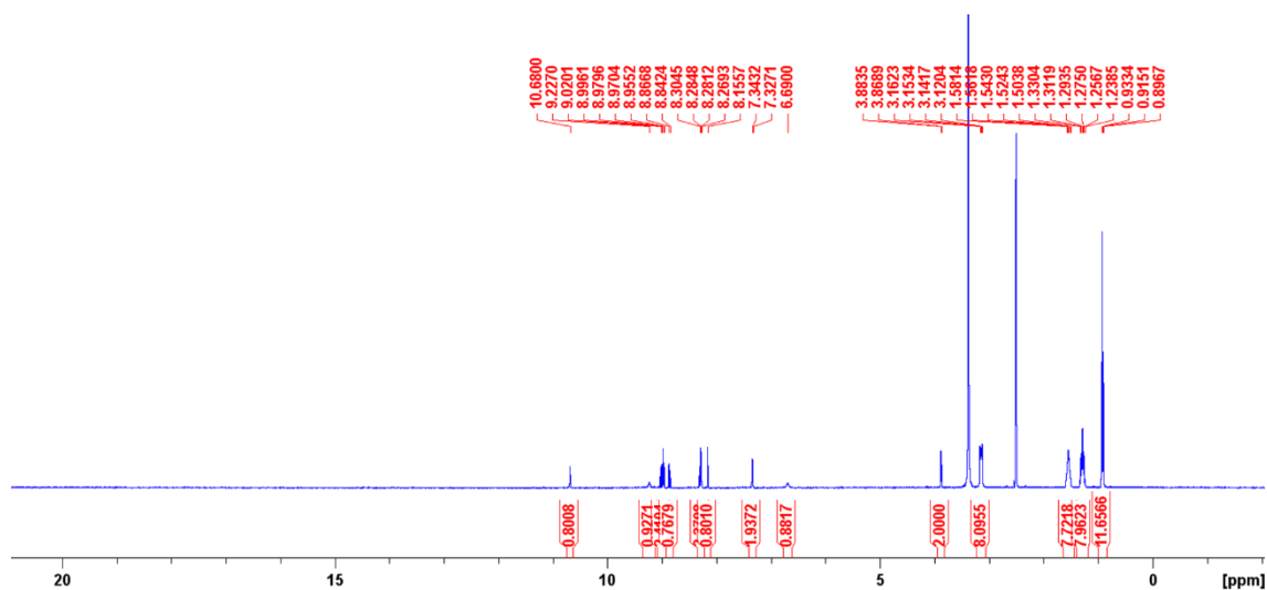
Figure S18 - 1 H NMR of compound Co-formulation g in DMSO- d 6 conducted at 298 K.
