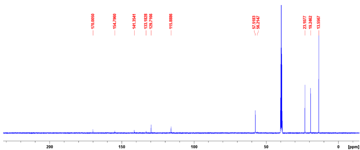
Figure S9 - 13 C{ 1 H} NMR of compound 5 in DMSO- d 6 conducted at 298 K
