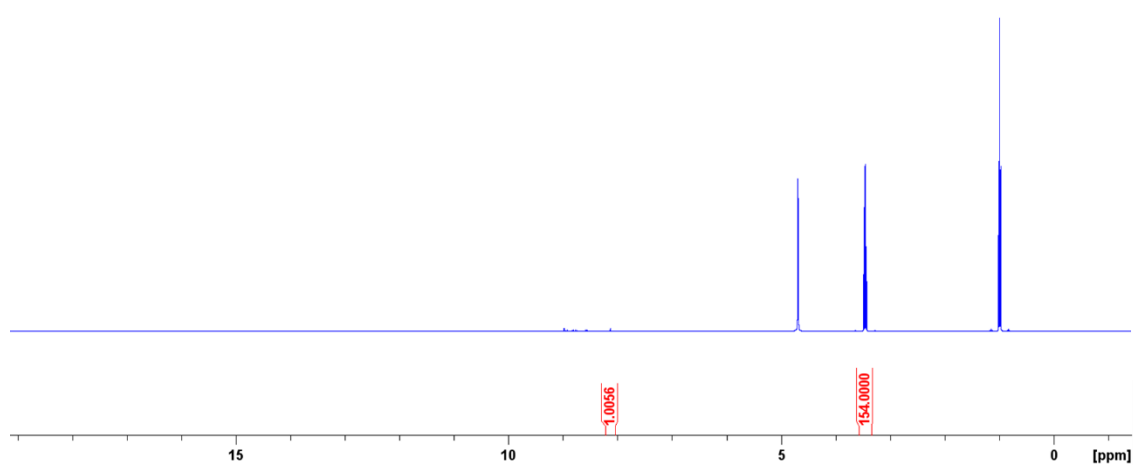
Figure S38 - ^1\text{H} NMR spectrum with a delay ( d_1 = 60 s) of 7 (11.12 mM) in \text{D}_2\text{O}/5.0\% EtOH. Comparative integration indicated 0% of sample has become NMR silent.
