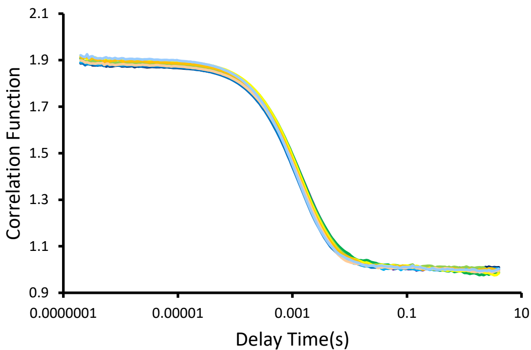
Figure S90 - Correlation function data for 10 DLS runs of 5 + 8 (5.56 mM) in a EtOH/H 2 O 1:19 solution at 298 K.
