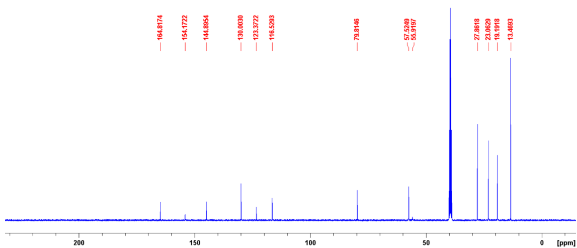
Figure S7 - 13 C{ 1 H} NMR of compound 4 in DMSO- d 6 conducted at 298 K
