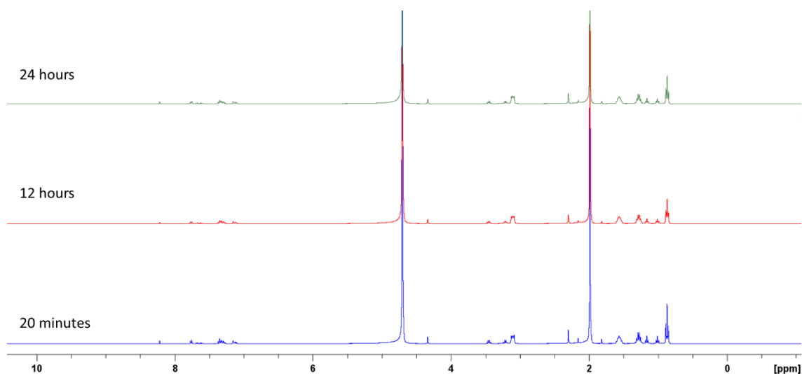
Figure S51 - Zoomed in 1 H NMR spectrum with a delay ( d_1 = 60 s) of Co-formulation I (5.56 mM) in D 2 O/1.0% CH 3 CN. Comparative integration indicated 23% of sample has become NMR silent 20 minutes after the addition of N, N-Diethyl-meta-toluamide, 26% of the sample has become NMR silent after 12 hours and 30% has become NMR silent after 24 hours.
