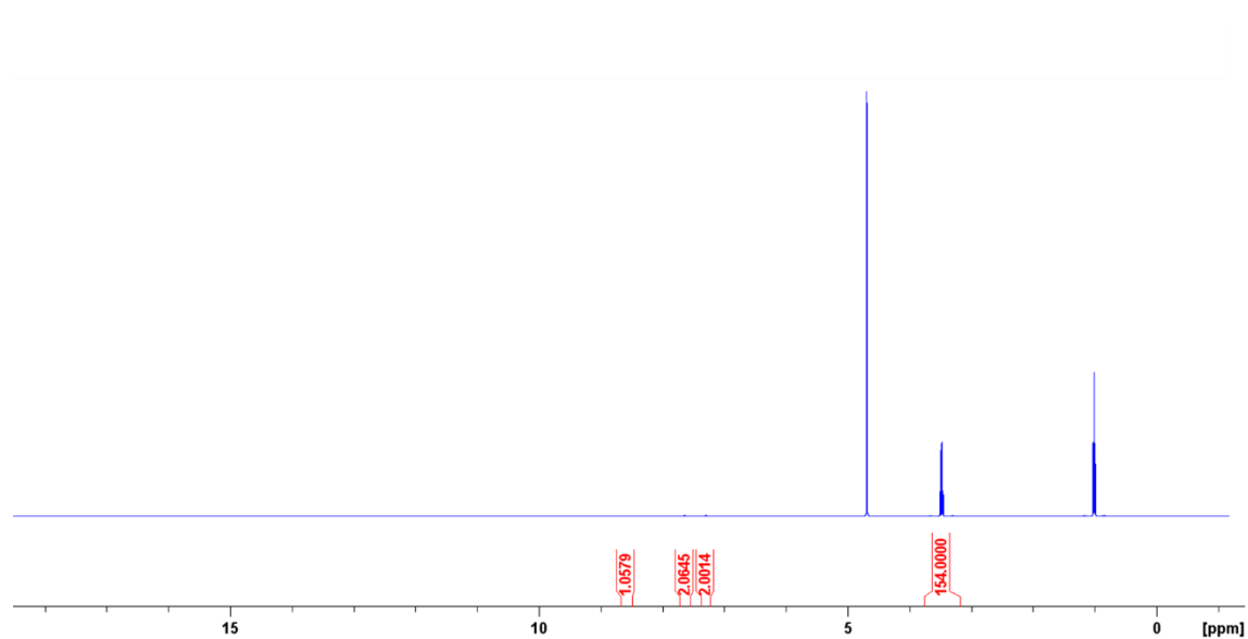
Figure S37 - ^1\text{H} NMR spectrum with a delay ( d_1 = 60 s) of 6 (11.12 mM) in \text{D}_2\text{O}/5.0\% EtOH. Comparative integration indicated 0% of sample has become NMR silent.
