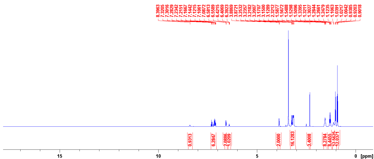
Figure S21 - 1 H NMR of compound Co-formulation j in DMSO- d 6 conducted at 298 K.
