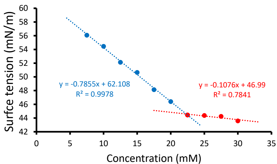
Figure S117 - Calculation of CAC (21.38 mM) for compound Co-formulation i in a H 2 O solution using surface tension measurements.
