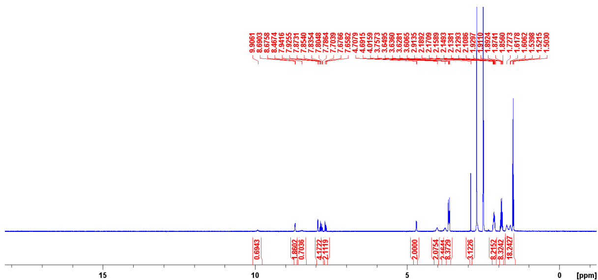
Figure S22 - 1 H NMR of compound Co-formulation k in DMSO- d 6 conducted at 298 K.
