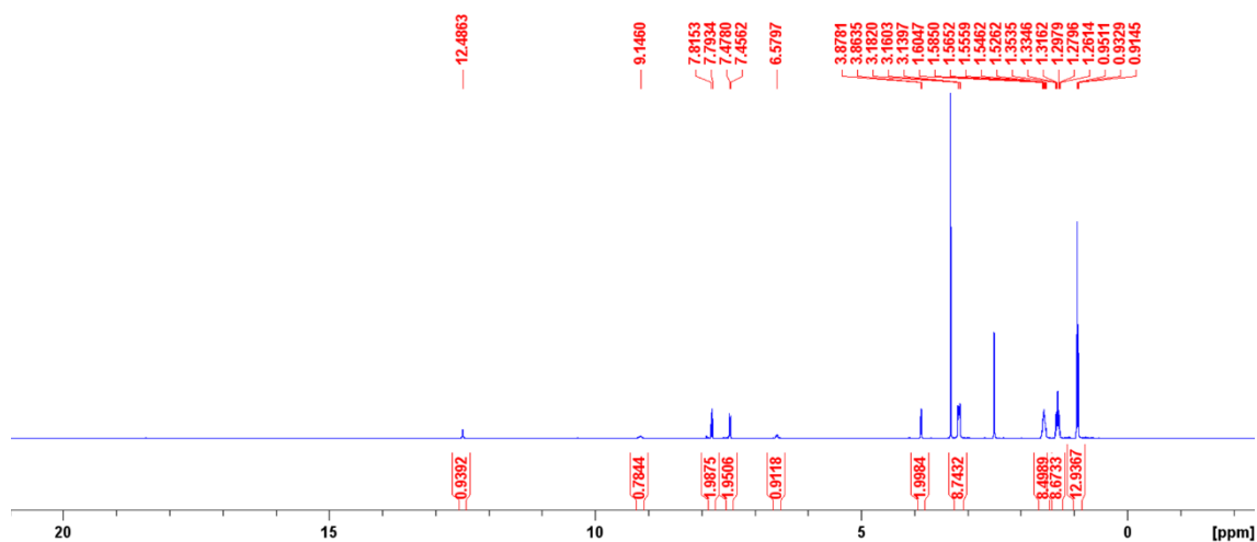
Figure S8 - 1 H NMR of compound 5 in DMSO- d 6 conducted at 298 K.
