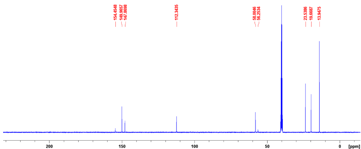
Figure S5 - 13 C{ 1 H} NMR of compound 3 in DMSO- d 6 conducted at 298 K
