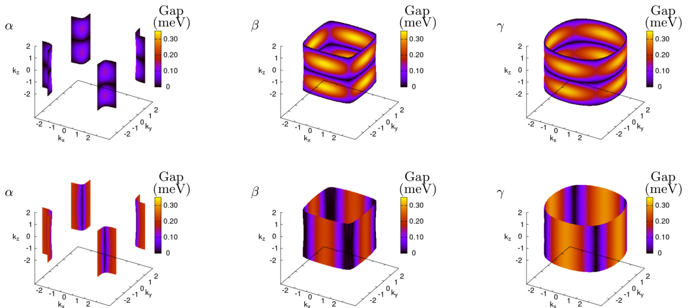
FIG. 1. (Color online) Variation of zero temperature superconducting gap on the three Fermi sheets of the normal state of \text{Sr}_2\text{RuO}_4 . The top (bottom) row is for the E_g ( B_{1g} ) pairing. Whereas the E_g pairing has horizontal line nodes at k_z = 0, \pm 2\pi/c , B_{1g} has vertical line nodes at k_x = \pm k_y . k_x, k_y and k_z are in units of the in-plane lattice constant a = 3.862 \text{ \AA} . c = 12.722 \text{ \AA} is the lattice constant along z -axis.
