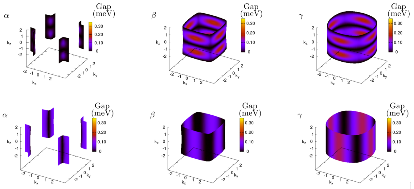
FIG. 9. (Color online) Superconducting gap plotted at a field of 2.67 Tesla on the normal state Fermi surface. The upper row is for E_g pairing while lower row is for B_{1g} pairing. Note that for the more two-dimensional nature of the B_{1g} pairing the superconducting gap is significantly suppressed on the \alpha and \beta sheets (of dominantly out-of-plane d_{xz} and d_{yz} character) as compared to the \gamma sheet (of dominantly in-plane d_{xy} character). In contrast for the E_g pairing the gap size is comparable on all three Fermi sheets.
