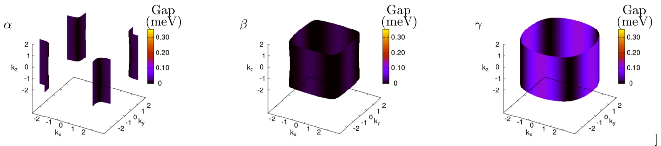
FIG. 10. (Color online) Superconducting gap plotted at a field of 2.97 Tesla on the normal state Fermi surface for B_{1g} pairing. Whereas the superconducting gap has almost vanished on the \alpha and \beta cylinders, the \gamma sheet remains superconducting.
