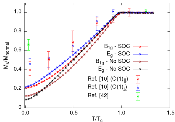
FIG. 4. (Color online) Temperature variation of the ratio of spin moment in the superconducting and normal state at \sim 0.7 T for d_{xz} + id_{yz} ( E_g ) and d_{x^2-y^2} ( B_{1g} ) pairing. Shown also is the same data with spin orbit coupling (SOC) switched off. Experimental data for the Knight shift at 0.7T from NMR measurements and PNS data at 0.5 T are also shown for comparison.
