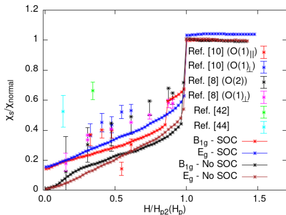
FIG. 5. (Color online) Spin susceptibility ratio as a function of field for temperature value of 25 mK for d_{xz} + id_{yz} ( E_g ) and d_{x^2-y^2} ( B_{1g} ) pairing. Also presented is experimental data for the Knight shift measured at two different positions of Oxygen atoms at 66 mK [10] and at 25 mK [8] and the PNS data at 60 mK [42] and at 25mK [44]. Note that the applied magnetic field has been divided by the critical field value H_p , which for the case of d_{x^2-y^2} is chosen to be the upper critical field H_{p2} , see the discussion of the H - T phase diagram in Sec. IV C.
