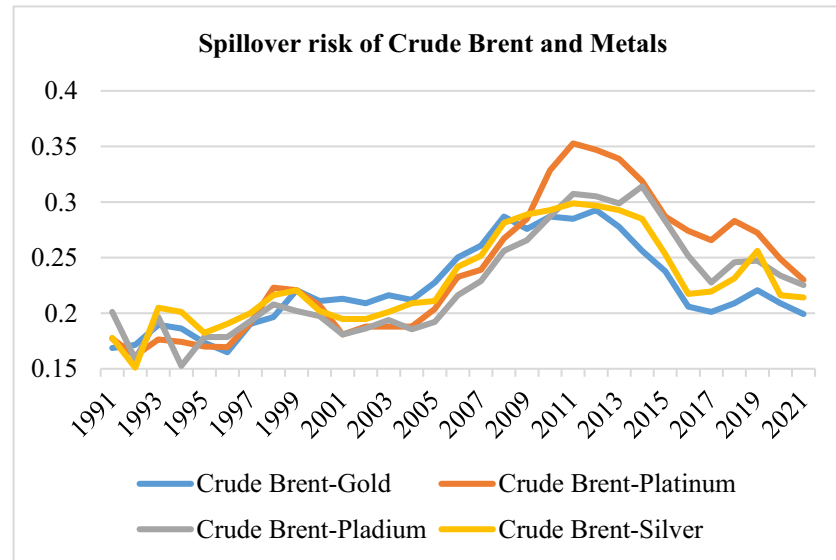
Fig. 3. The rolling spillover risk of crude oil and precious metals.
