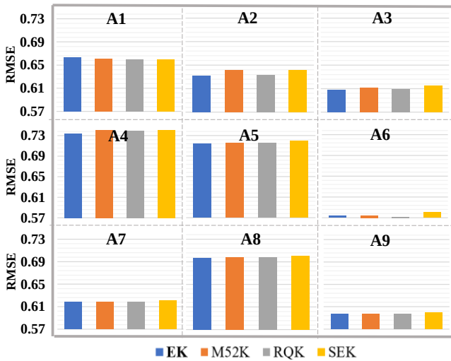
Fig. 5. Comparison of RMSE for four GPR models with different kernel functions.
