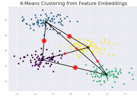
Fig. 2: Identifying Reference Points (illustration): We apply k-means over the dataset of domestic sounds. The red dots represent the mid points between cluster centres. We select the 3 points with the lowest density.
