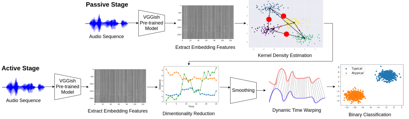
Fig. 1: Pipeline: The process aims to analyse a stream of sounds captured over a long time window where the user performs a typical routine (e.g. morning routine) and compares the sound patterns with previously captured “normal” routine for that individual. The process does not rely on the identification of the specific activities, and therefore does not require labeled data for training.
