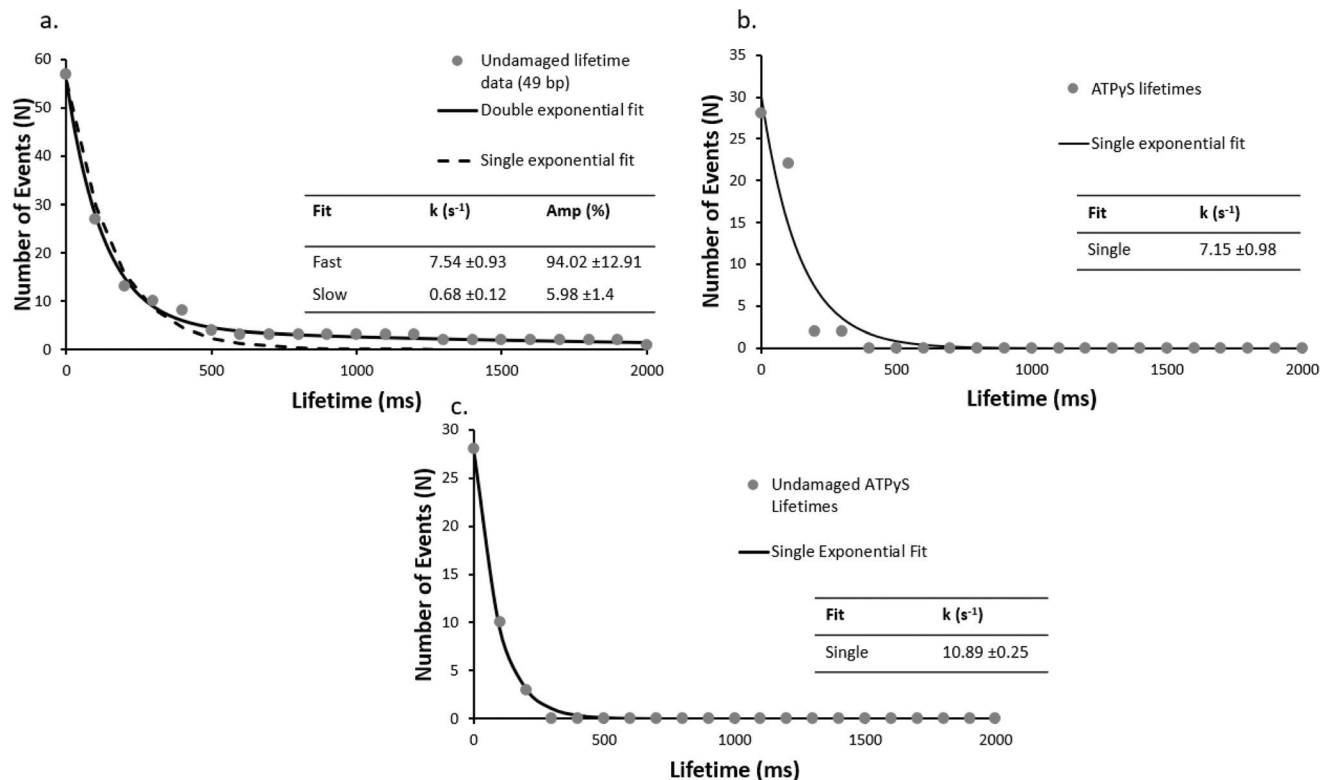
Fig. 3 DNA length has no impact on fast lifetimes, but in the presence of ATP \gamma S UvrA loses the slow phase. Cumulative decay plots with a shorter (undamaged_49 bp) undamaged DNA construct (a), are unchanged kinetically from the 98 bp construct suggesting the lifetimes are not limited by sliding off the DNA ( r^2 = 0.98 vs. 0.55 , for double and single exponential fit respectively). UvrA interactions were also studied on (b) 98 bp damaged DNA (damaged_98 bp) and (c) 98 bp undamaged DNA (undamaged_98 bp) in the presence of 1 mM ATP \gamma S where no slow events were seen. The observed interactions fit well to a single exponential with a detachment rate constant of 7.15 \text{ s}^{-1} and 10.89 \text{ s}^{-1} for damaged and undamaged DNA respectively ( r^2 = 0.99 and 0.91 for single exponential fit on undamaged and damaged DNA respectively).
