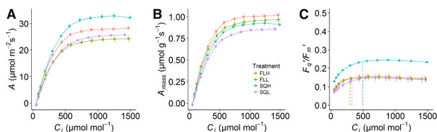
Figure 4. Photosynthesis as a function of C_i of plants grown under the four light treatments SQH, FLH, SQL, and FLL. Parameters examined are A (A), A_{mass} (B), and F_q'/F_m' (C). Data represent means \pm SE ( n = 6 ).
