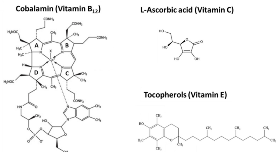
Figure 5. The chemical structures of Vitamin B 12 (pyrrole rings are labelled A to D); Vitamin C and Vitamin E.
