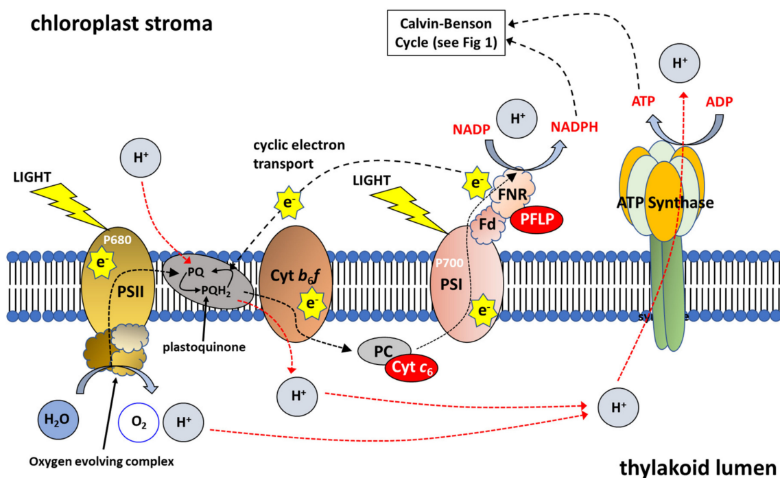
Figure 2. Schematic Representation of Photosynthetic Electron Transport. Photosystem I (PSI), Photosystem II (PSII), Cytochrome b_6/f complex (Cyt b_6/f ), plastocyanin (PC), Ferredoxin (Fd) and ferredoxin-NADP reductase (FNR). Cytochrome c_6 (Cyt c_6 ) transfers electrons from the Cyt b_6/f complex to PSI at a faster rate than observed for PC; plant ferredoxin-like protein (PFLP) (Adapted from [23]).
