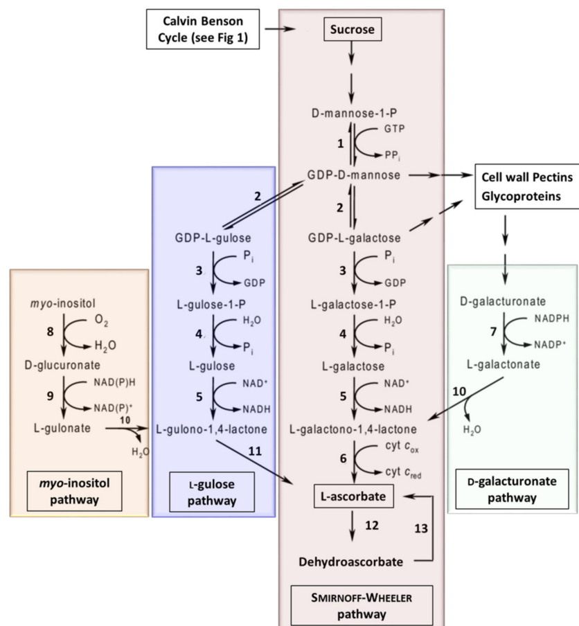
Figure 6. The biosynthetic pathways for vitamin C in plants. Enzymes: 1, GDP-D-Man pyrophosphorylase; 2, GDP-Man-3',5'-epimerase; 3, GDP-L-Gal phosphorylase (or transferase); 4, L-Gal 1-phosphate phosphatase; 5, L-Gal dehydrogenase; 6, L-GalL dehydrogenase; 7, D-galacturonate reductase; 8, myo-inositol oxygenase; 9, D-glucuronate reductase; 10, aldono-lactonase; 11, L-GulL oxidase (or dehydrogenase); 12, ascorbate oxidase; 13, dehydroascorbate reductase (adapted from [149,208]).
