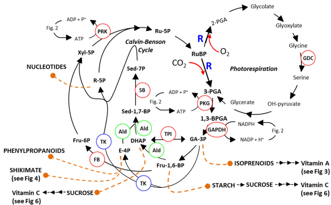
Figure 1. Schematic Representation of Photosynthesis and Photorespiration. Sedoheptulose-1,7-bisphosphatase (SB: EC.3.1.3.37), fructose-1,6-bisphosphate aldolase (Ald: EC.4.1.2.13), fructose-1,6-bisphosphatases (FB: EC.3.1.3.11), triosephosphate isomerase [TPI: EC 5.3.1.1], transketolase (TK: EC.2.2.1.1), phosphoribulokinase (PRK: EC.2.7.1.19), phosphoglycerate kinase (PKG: EC.2.7.2.3), ribulose-bisphosphate carboxylase (R: EC.4.1.1.39), Glyceraldehyde-3-phosphate dehydrogenase (GAPDH) and Glycine decarboxylase (GDC). (see [39]).
