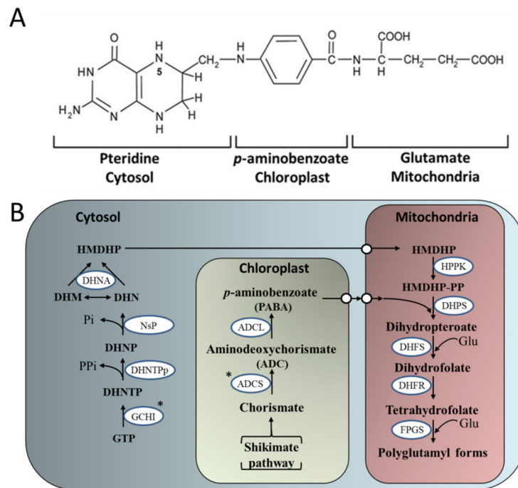
Figure 4. The plant folate biosynthesis pathway. (A) The chemical structure of monoglutamyl tetrahydrofolate (B) The pteridine pathway leading to hydroxymethyldihydropterin (HMDHP) in the cytosol; the pathway leading to p-aminobenzoate in the plastid, and condensation steps localized in the mitochondria are shown. DHN, dihydroneopterin; -P, monophosphate; -PP, pyrophosphate; -PPP, triphosphate; DHM, dihydromonapterin; Glu, glutamate; ADCS, aminodeoxychorismate synthase; ADCL, aminodeoxychorismate lyase; GCHI, GTP cyclohydrolase I; DHNTpp, dihydroneopterin triphosphate pyrophosphatase; NsP, non-specific phosphatase; DHNA, dihydroneopterin aldolase; HPPK, hydroxymethyldihydropterin pyrophosphokinase; DHPS, dihydropteroate synthase; DHFS, dihydrofolate synthase; DHFR, dihydrofolate reductase; FPGS, folylpolyglutamate synthetase. White circles represent points of substrate transport. *targeted enzymes for over-expression (Adapted from [155,156]).
