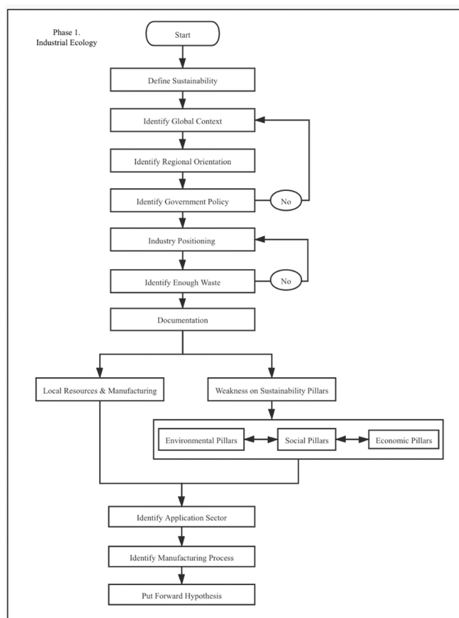
Figure 3. The process of conducting an industrial ecology study.
