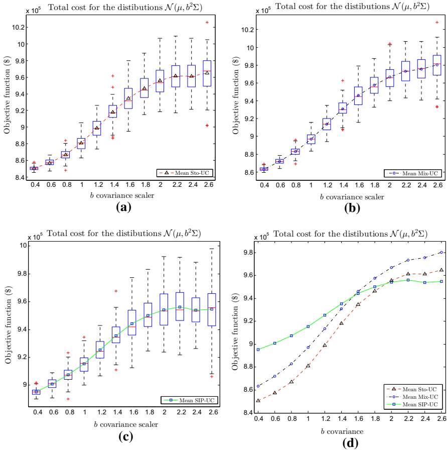
Fig. 4 Sensitivity of solutions to variation in covariance. a Sto-UC. b Mix-UC. c SIP-UC. d Mean objective values for 100 runs
