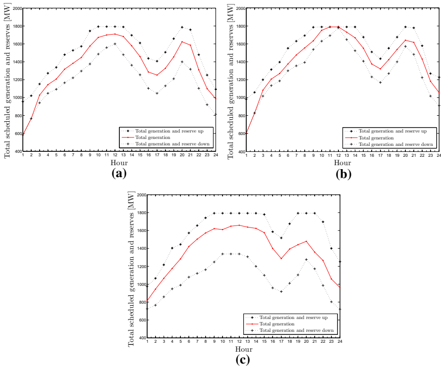
Fig. 2 UC first-stage solutions. a Sto-UC. b Mix-UC. c SIP-UC
