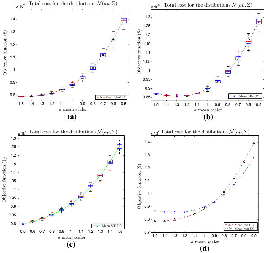
Fig. 3 Sensitivity of solutions to variation in mean. a Sto-UC. b Mix-UC. c SIP-UC. d Mean objective values for 100 runs
