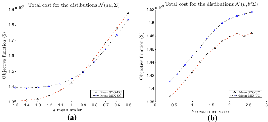
Fig. 7 Sensitivity of solutions to variation in mean and variance for a medium-sized problem with 100 generators (with T = 12, S = 150 ). a Mean objective values for 100 runs. b Mean objective values for 100 runs
