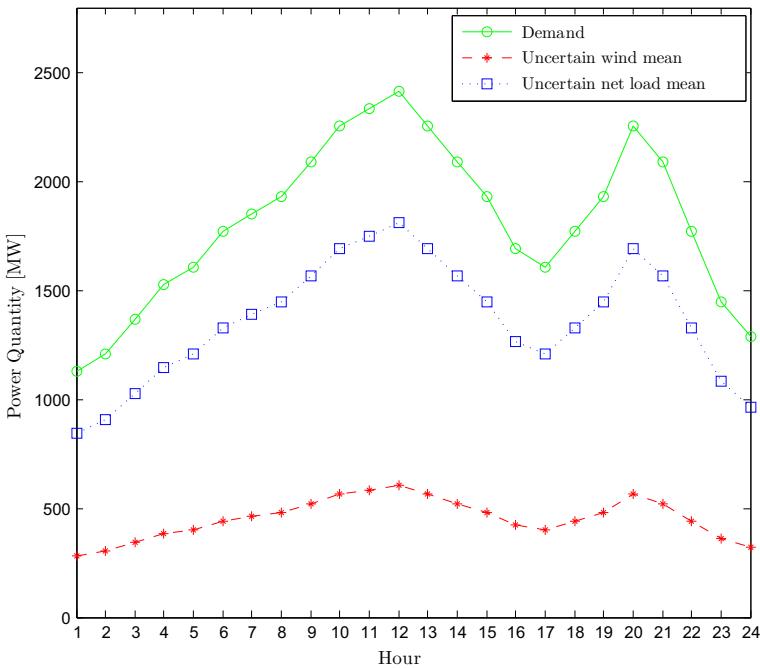
Fig. 1 Nominal values of demand and mean wind
