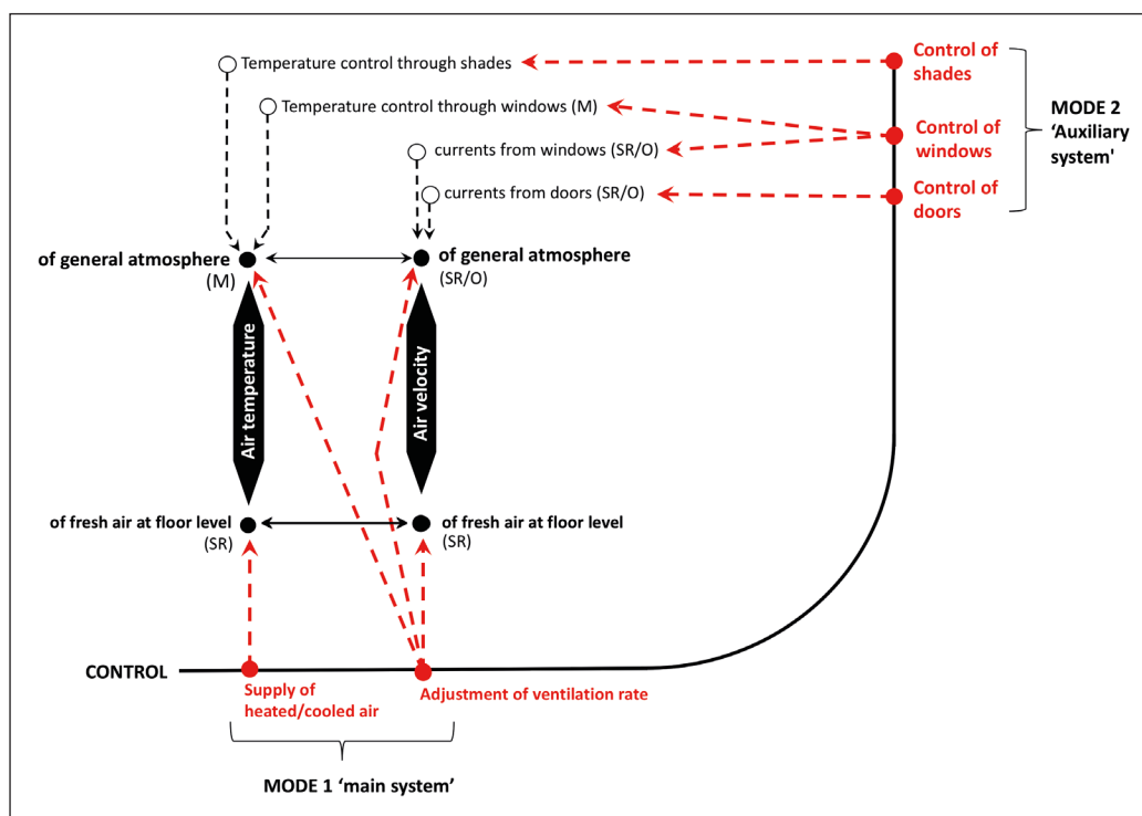
Figure 9: Socio-technical control and feedback system. Note: M = measurements; O = direct observation by staff and officials; and SR = user feedback. Source: Author’s own drawing.
