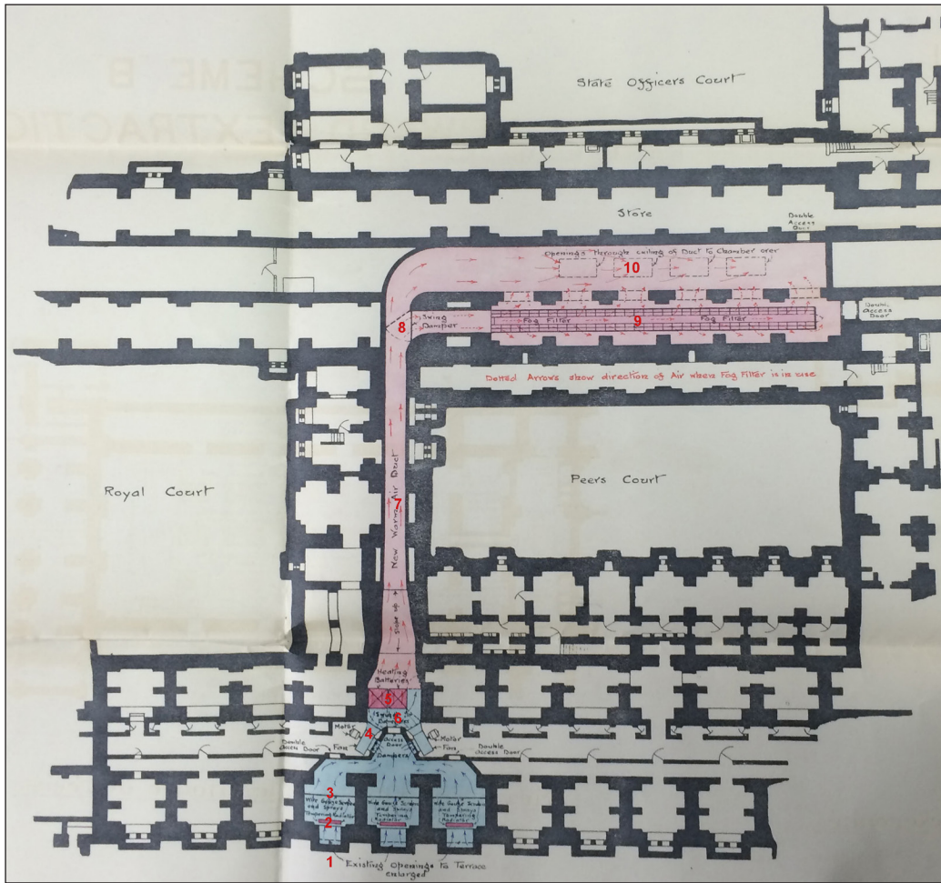
Figure 11: Floor plan of the scheme for new air intake, 1912.
