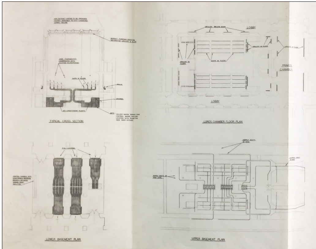
Figure 14: Proposed air-conditioning system, November 1963, show ductwork and the configuration of floor grills. Source: National Archives, Work 11 Series, Box 588.
