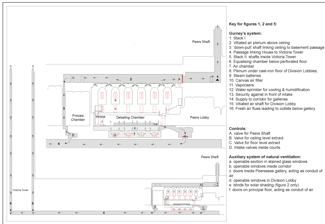
Figure 1: Houses of Parliament: diagrammatic cross-section showing the stack ventilation system with control valves.
