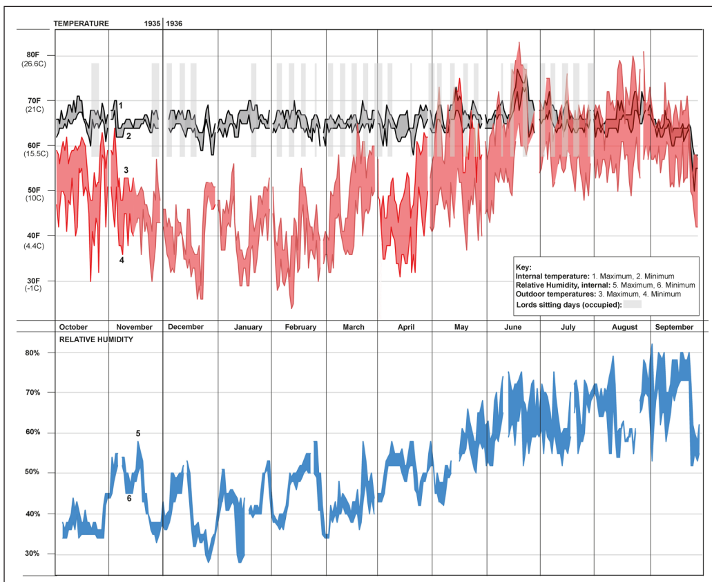
Figure 12: Temperature and humidity recorded inside the House of Lords, October 1935 and September 1936.
