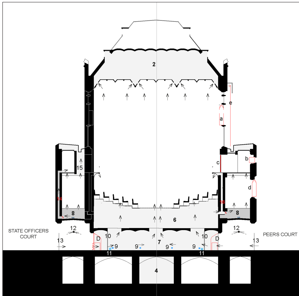
Figure 2: Cross-section showing features of the environmental system.
