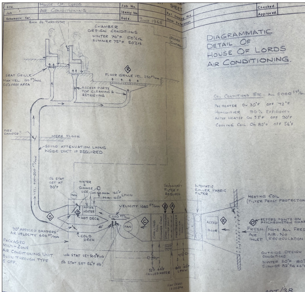
Figure 15: Sketch of the mock-up system, June 1965. Source: Ministry of Public Building and Works (1965).
