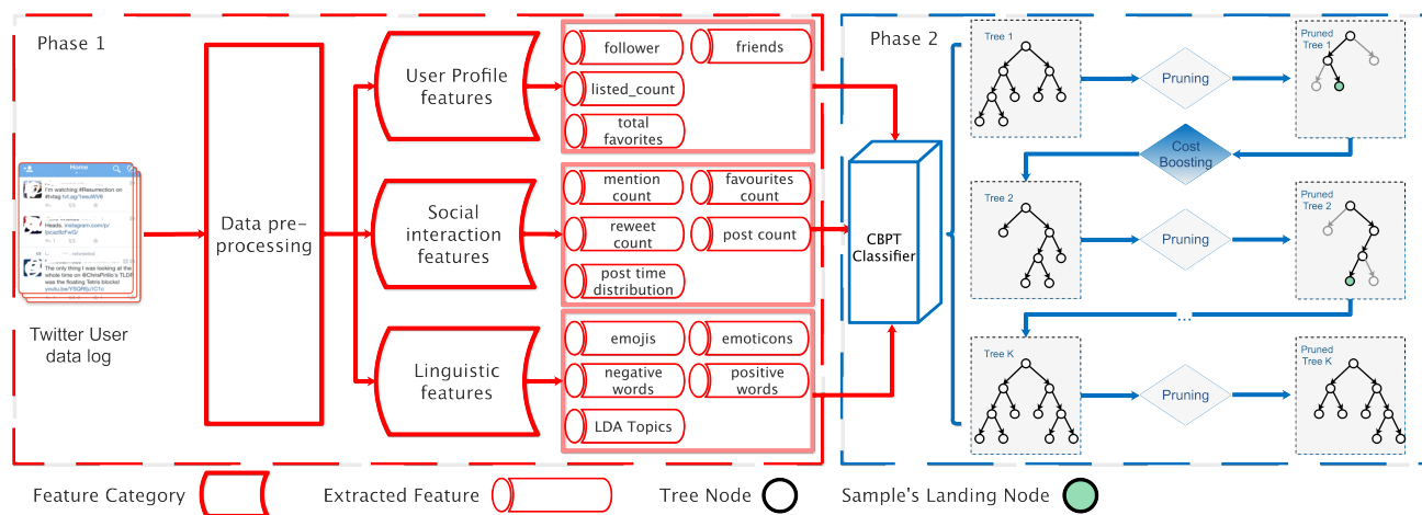
Fig. 1: Proposed framework. In phase 1, we conduct data preprocessing and extract various discriminative features of Twitter users. In phase 2, the CBPT classifier combines the power of K pruned trees. The cost-sensitive boosting structure relies on the landing position of samples in the pruned tree structure and an example of the sample decision path is highlighted in dark black in the diagram.
