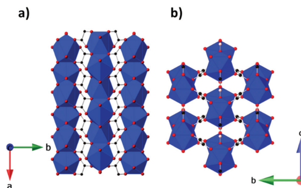
Fig. 11 (a) Crystal structure of Ln(HCO 2 )(C 2 O 4 ) with infinite one-dimensional chains grow along the a -axis. (b) Arrangement of the chains in a triangular lattice on the bc -plane. Colour codes: Ln: blue, C: black, O: red, H: pink.
