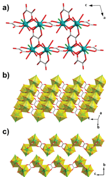
Fig. 10 Crystal structure of Gd(C 2 O 4 )(H 2 O) 3 Cl, with (a and b) 2D layers on the ac -plane and (c) packing along the b -axis. Colour codes: Gd: cyan, C: grey, O: red. The hydrogen atoms have been omitted for clarity. Adapted with permission from Inorg. Chem. , 2014, 53(17), 9052–9057. Copyright 2014 American Chemical Society.
