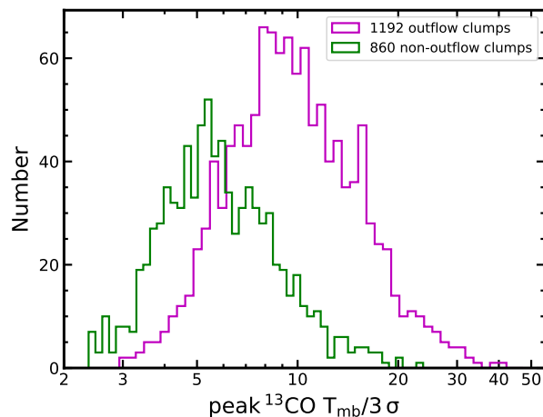
Fig. 7. The distribution of the ratio between the peak intensity of the 13 CO line and the 3 \sigma detection level of the corresponding spectrum for the outflow sample (magenta histogram) and the non-outflow sample (green histogram).
