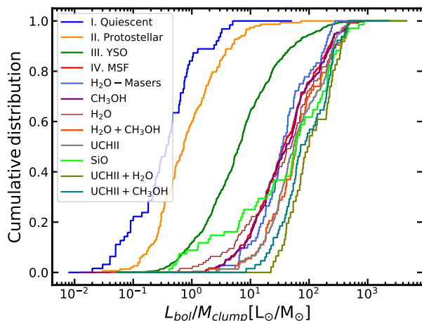
Fig. 8. Top-panel: outflow detection rate of clumps in different evolutionary stages and associated with different star-forming activities, as presented in Table 4. The error bars of each group are calculated from the binomial errors and the error of the detection rate for clumps with HCH II regions is adopted from the binomial errors of the total clump sample. Bottom-panel: cumulative distributions of luminosity-to-mass ratios ( L_{\text{bol}}/M_{\text{clump}} ) for the subsamples of outflow clumps in the top panel, which indicate the evolutionary stages of these subsamples.
