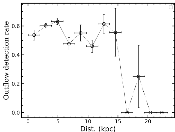
Fig. 6. The outflow detection rate as a function of clumps’ heliocentric distances (Dist.), showing that the detection rates are more or less similar for clumps with Dist. < 14 kpc, and quickly decrease in clumps with Dist. > 14 kpc. As <1% of sources in the sample have Dist. > 14 kpc, any distance bias wouldn’t significantly impact the statistical analysis of the outflow detection in this work. The error bars on the x-axis are derived the bin size of distances and y-axis are calculated from the standard error of binomial distribution of the detection rate, as shown in Sect. 4.1.
