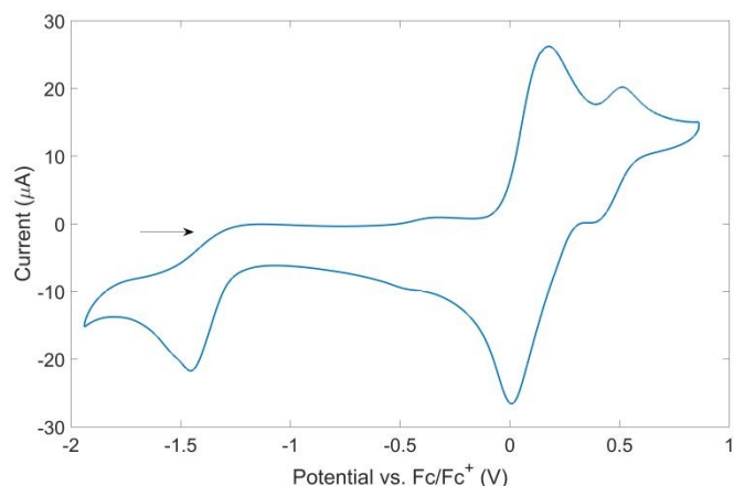
Figure 6. Cyclic voltammogram of 2a in DCM with [t\text{Bu}_4\text{N}][\text{PF}_6] supporting electrolyte.
