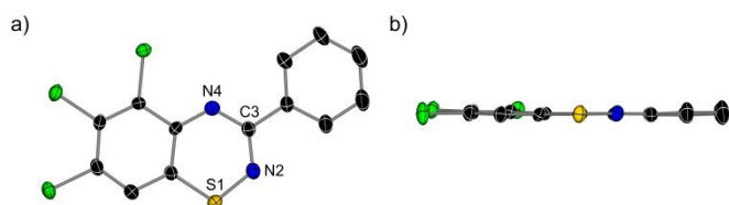
Figure 3. Molecular structure of [4a][GaCl 4 ] . Thermal ellipsoids shown at 50% probability. Hydrogen atoms and counter-anion omitted for clarity. a) Top-down view; b) Side view.
