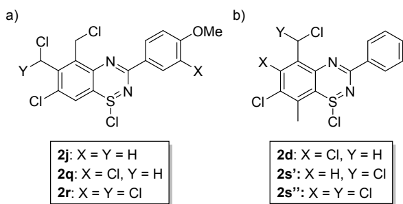
Figure 1. Partially chlorinated 1,2,4-benzothiadiazine 1-chlorides derived from 1j and 1d .
