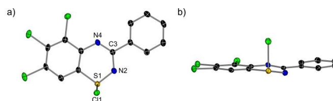
Figure 2. Molecular structure of 2a . Thermal ellipsoids shown at 50% probability. Hydrogen atoms omitted for clarity. a) Top-down view; b) Side view.
