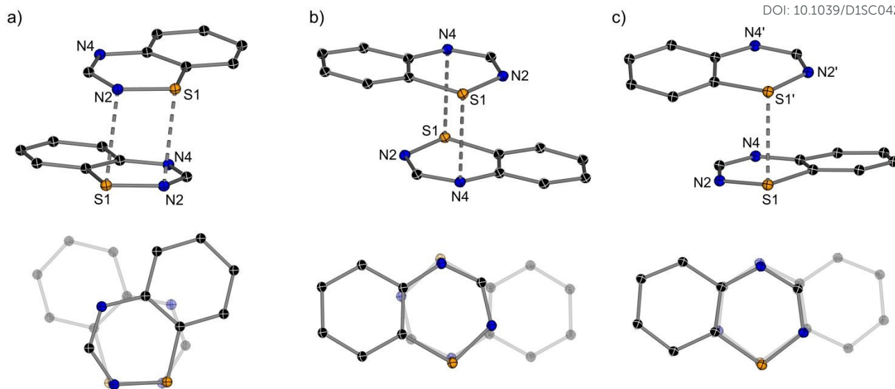
Figure 7. Dimerisation motifs, shown as side-on and top-down views, observed for 1,2,4-benzothiadiazinyl radicals: a) 3a - suprafacial; b) 3c and 3k - trans -antarafacial; c) 3e - trans -suprafacial. The pendant aryl ring and substituents on the benzo-fused ring have been omitted for clarity.
