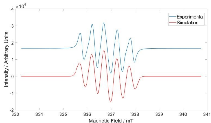
Figure 4. EPR spectra of 3a .
