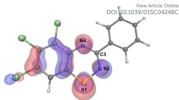
Figure 5. Calculated SOMO of 3a (isovalue = 0.04).
