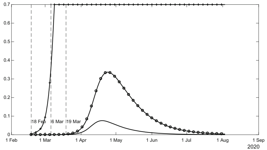
Fig. 4 Equilibrium social distancing against infections. The vertical dash lines indicate the dates 18 February, 6 March and 19 March. The plain solid line depicts infections as a percentage of the UK population, while the circle line shows the social distancing of low-risk individuals and the cross line the social distancing of high-risk people
