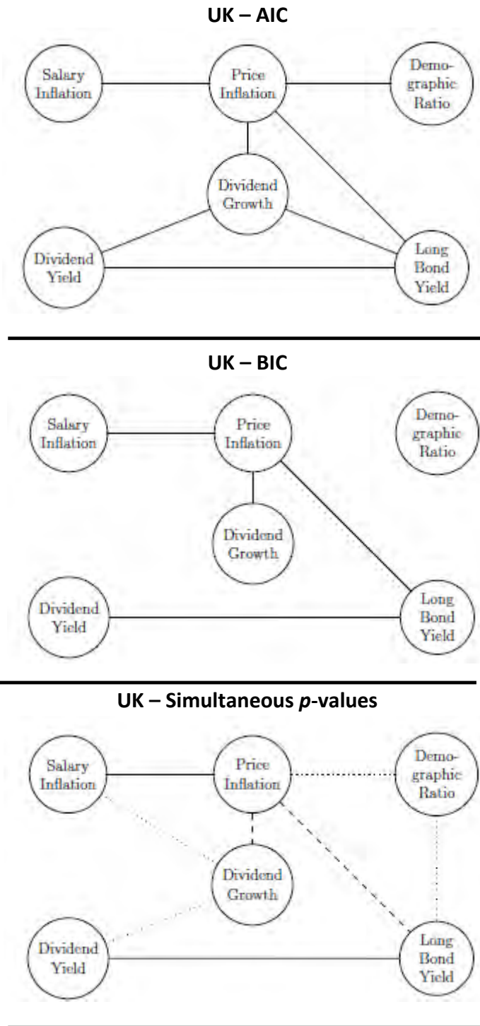
Figure 5: Alternative graphical model structures for the UK
