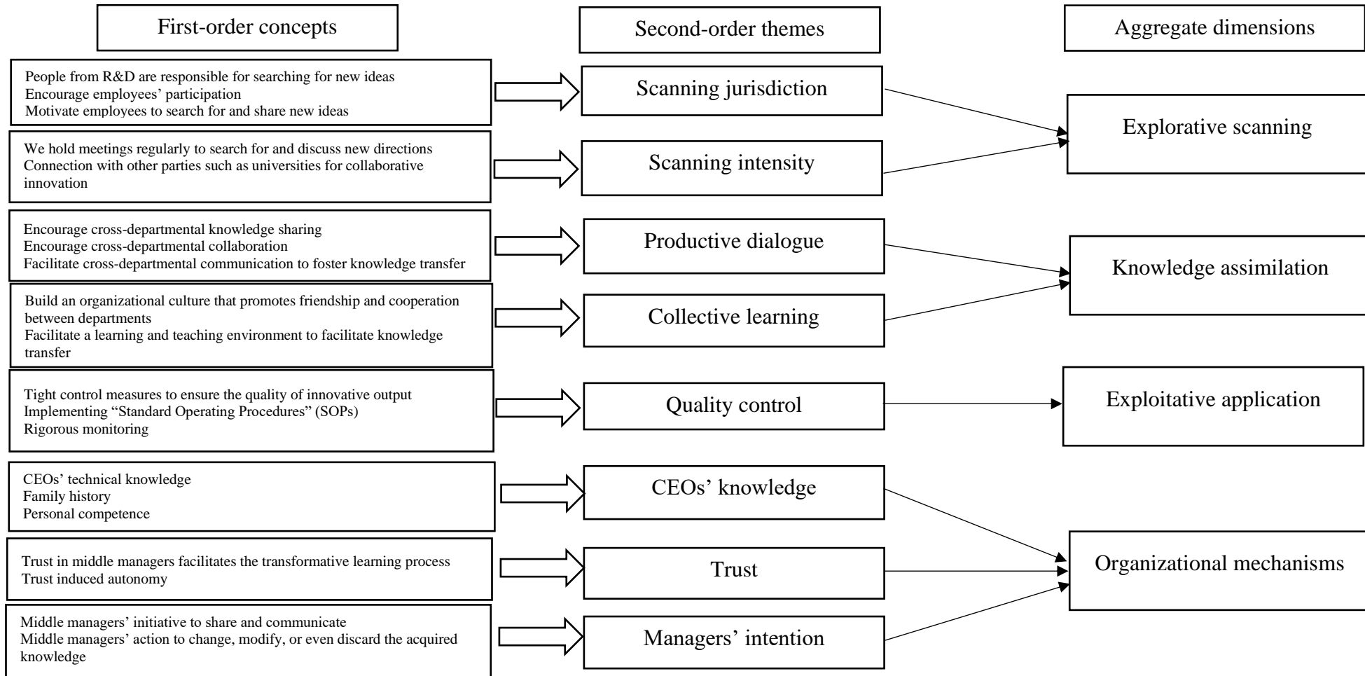
Figure 1. Data Structure
