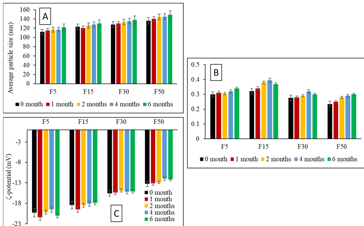
Figure 10. Effect of storage at 4 ± 1 °C on mean particle size (A), PDI (B) and ζ-potential (C) of OLZ-NLC formulations.
