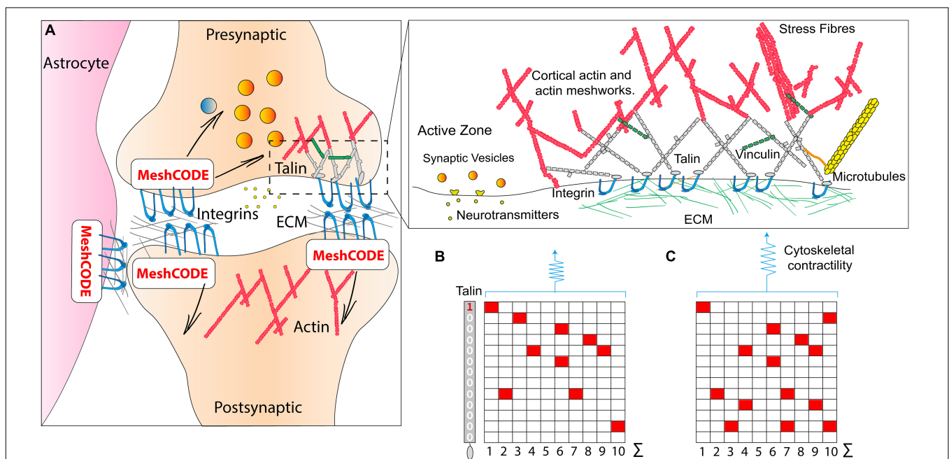
FIGURE 3 | The MeshCODE. (A) Schematic diagram of a tripartite synaptic junction. The integrin adhesion complexes and MeshCODEs in the presynaptic and postsynaptic zones, and in a neighbouring astrocyte are shown. The synapse is encapsulated by a specialised ECM that protects the mechanical environment of the MeshCODEs. Integrin and talin in one MeshCODE are shown connected to the actin cytoskeleton. (Right) Enlarged view of the highlighted region showing the MeshCODE intricately wired up to the cytoskeleton. Only the integrin-talin-actin adhesion core complex is shown, but up to 250 different proteins decorate this core dependent on the switch patterns of the talin scaffolds. The protein vinculin (green) binds to nine of the unfolded talin switch domains, stabilising them in the unfolded state and reinforcing the cytoskeletal connections. (B) A schematic of an array of ten talin molecules with the 13 switches arranged vertically. White, 0; red, 1. (C) Perturbations to the system result in changes in cytoskeletal contractility that alter the pattern of 1s and 0s written in the MeshCODE and its resultant output in a defined way.
