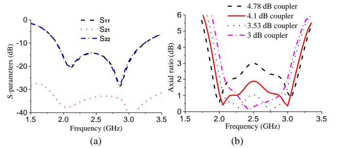
Fig. 6. (a) Simulated S-parameters of the dual-feed CP antenna without the feed network. (b) Simulated AR performances of the dual-feed CP antenna fed by different branch-line couplers.
