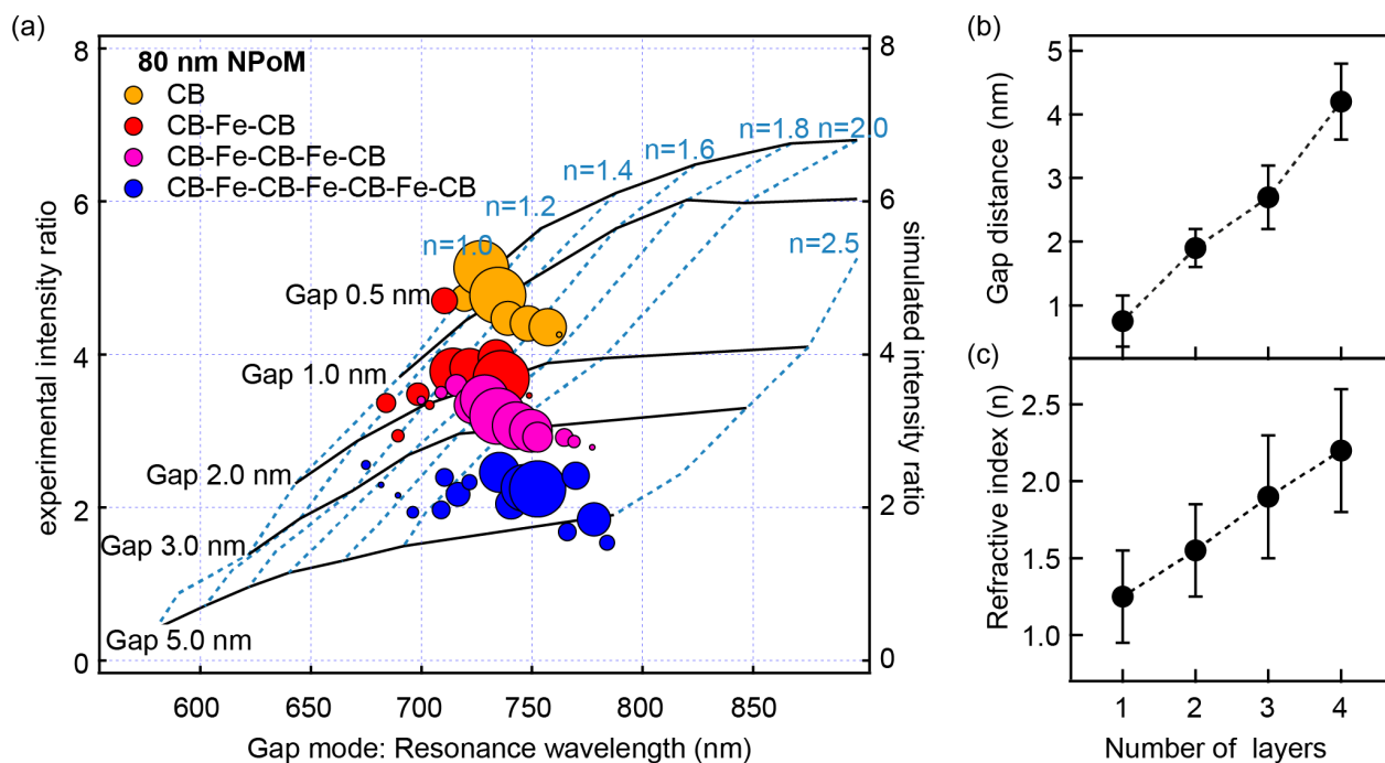
Fig. 4 (Left) Intensity ratios between coupled and transverse modes in NPoM geometries for CB[7], CB[7]·Fe 3+ ·CB[7], CB[7]·Fe 3+ ·CB[7]·Fe 3+ ·CB[7] and CB[7]·Fe 3+ ·CB[7]·Fe 3+ ·CB[7]·Fe 3+ ·CB[7] spacers plotted against the resonance wavelength with results obtained from Finite Difference Time domain (FDTD) simulations using different spacer thickness and refractive indices. (Right) Gap distance and refractive index plotted versus number of CB[7] layers.
