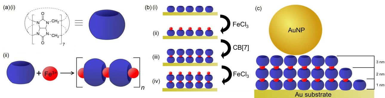
Fig. 1 (a)(i) The chemical structure of CB[7] is shown. (ii) A coordination complex forms when Fe 3+ and CB[7] are mixed in water. (b) Schematic of the layer-by-layer process used to build up coordination complexes of CB[7] and FeCl 3 •6H 2 O onto gold substrates. (c) An illustration highlighting that surface deposited CB[7]-Fe 3+ can be used to yield well defined spacings with nanometer control in plasmonic systems consisting of a gold film and a gold nanoparticle.
