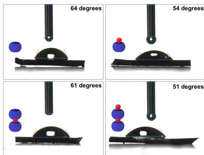
Fig. 3 Contact angle measurements highlighting the changes in hydrophobicity of a gold substrate after the layer-by-layer deposition of the CB-Fe 3+ nanostructure.
